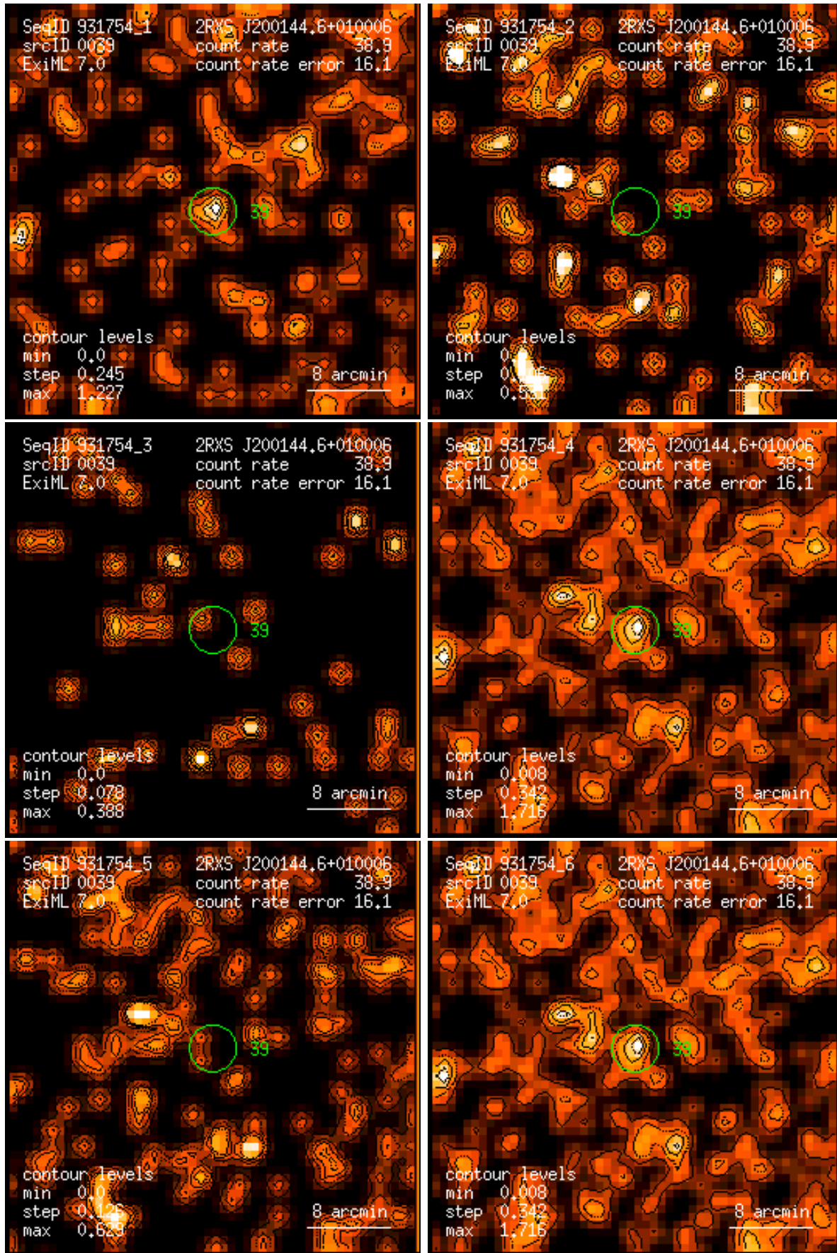
Figure 39: RASS 931754: detection 0039: band rate images, Gaussian filter: (1) PSPC channels 11 – 41, (2) 52 – 90, (3) 91 – 201, (4) 11 – 235, (5) 52 – 201, (6) 11 – 201. Broad band rates in counts/ks. Band rate contour levels in counts/ks/arcmin 2 .
