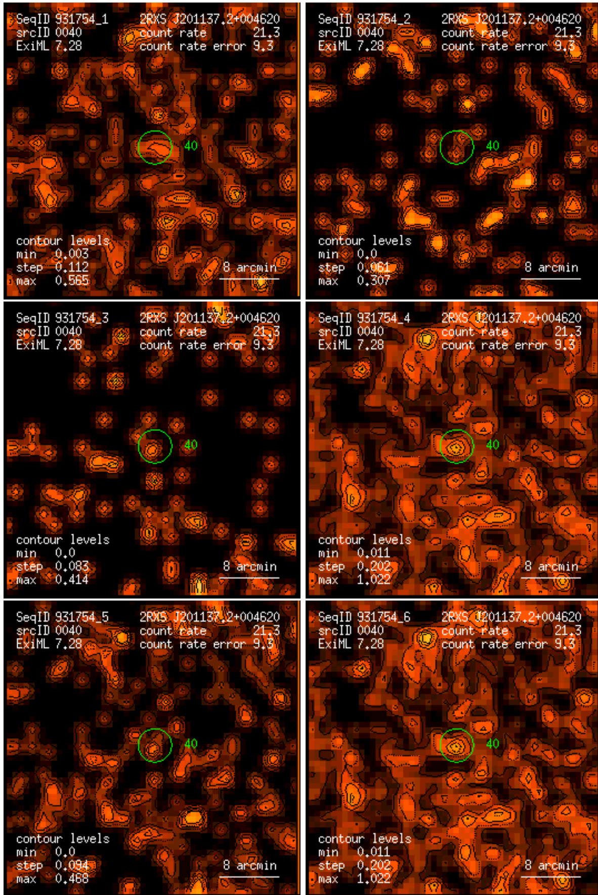
Figure 40: RASS 931754: detection 0040: band rate images, Gaussian filter: (1) PSPC channels 11 – 41, (2) 52 – 90, (3) 91 – 201, (4) 11 – 235, (5) 52 – 201, (6) 11 – 201. Broad band rates in counts/ks. Band rate contour levels in counts/ks/arcmin 2 .
