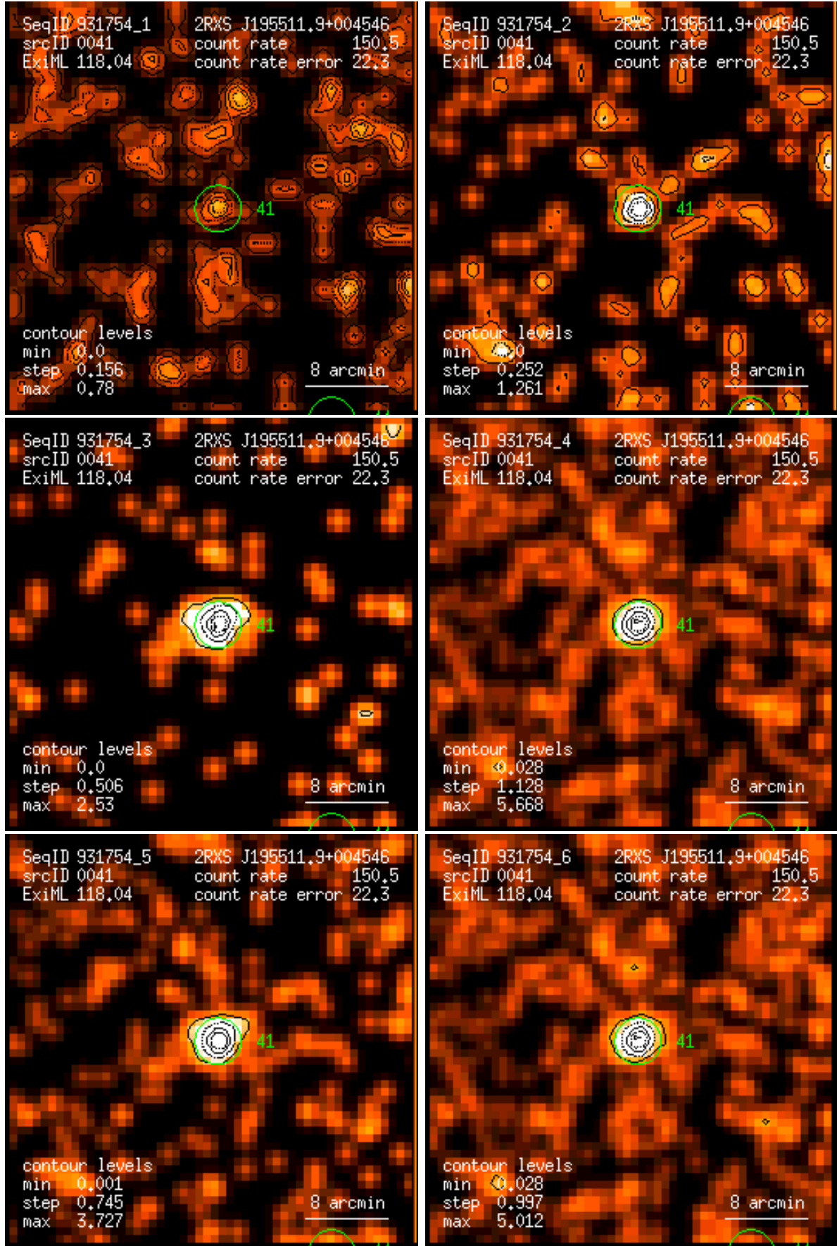
Figure 41: RASS 931754: detection 0041: band rate images, Gaussian filter: (1) PSPC channels 11 – 41, (2) 52 – 90, (3) 91 – 201, (4) 11 – 235, (5) 52 – 201, (6) 11 – 201. Broad band rates in counts/ks. Band rate contour levels in counts/ks/arcmin 2 .
