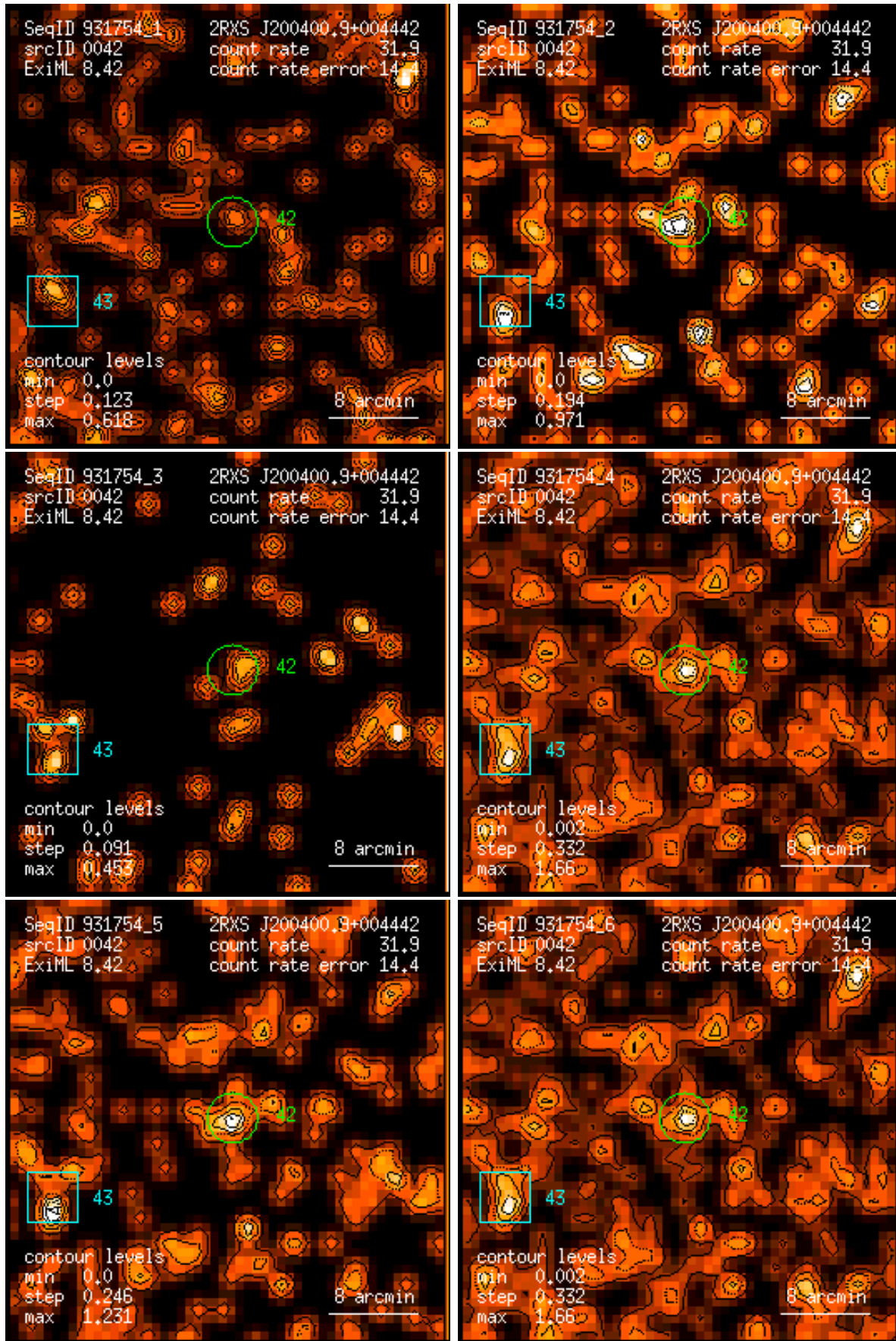
Figure 42: RASS 931754: detection 0042: band rate images, Gaussian filter: (1) PSPC channels 11 – 41, (2) 52 – 90, (3) 91 – 201, (4) 11 – 235, (5) 52 – 201, (6) 11 – 201. Broad band rates in counts/ks. Band rate contour levels in counts/ks/arcmin 2 .
