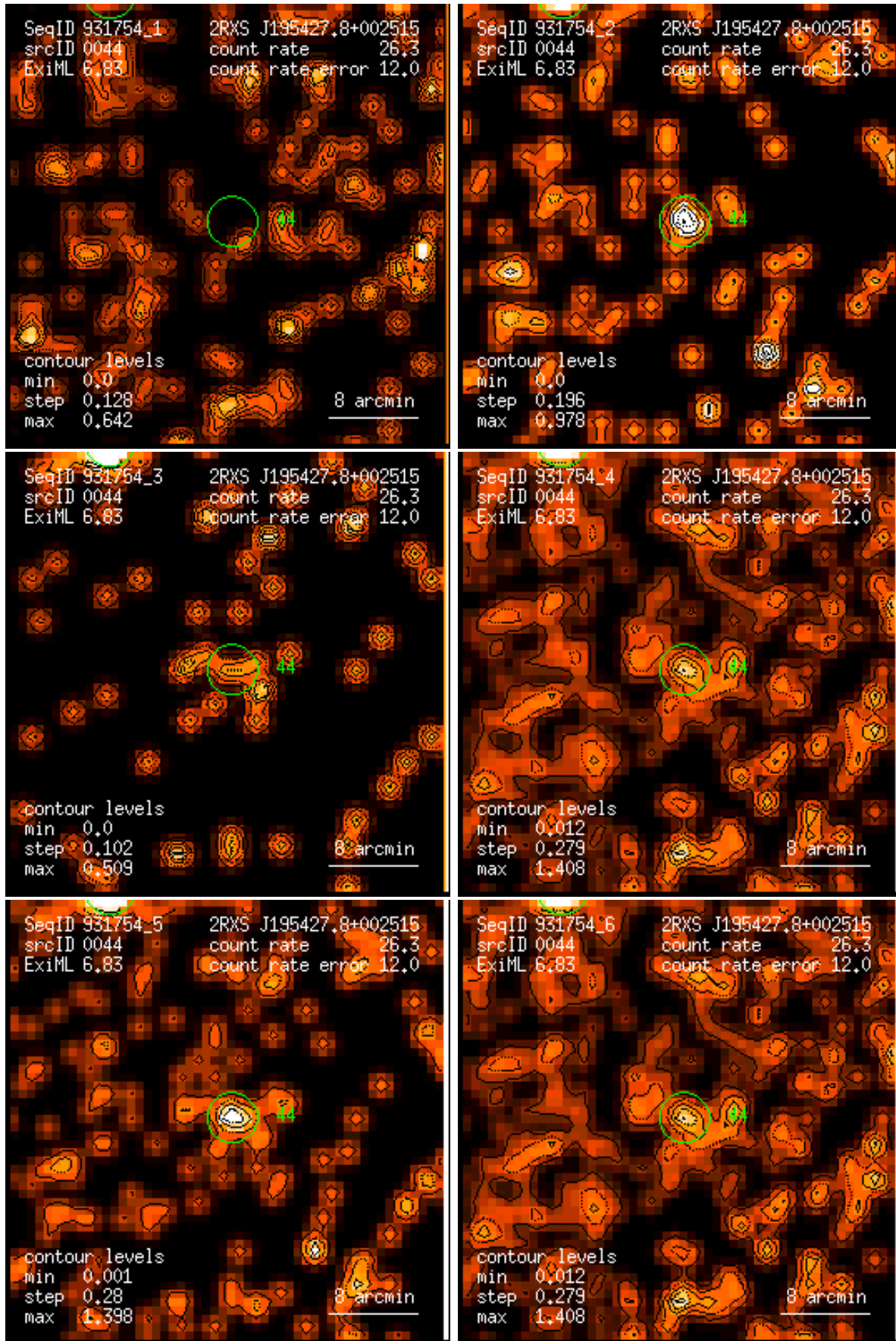
Figure 44: RASS 931754: detection 0044: band rate images, Gaussian filter: (1) PSPC channels 11 – 41, (2) 52 – 90, (3) 91 – 201, (4) 11 – 235, (5) 52 – 201, (6) 11 – 201. Broad band rates in counts/ks. Band rate contour levels in counts/ks/arcmin 2 .
