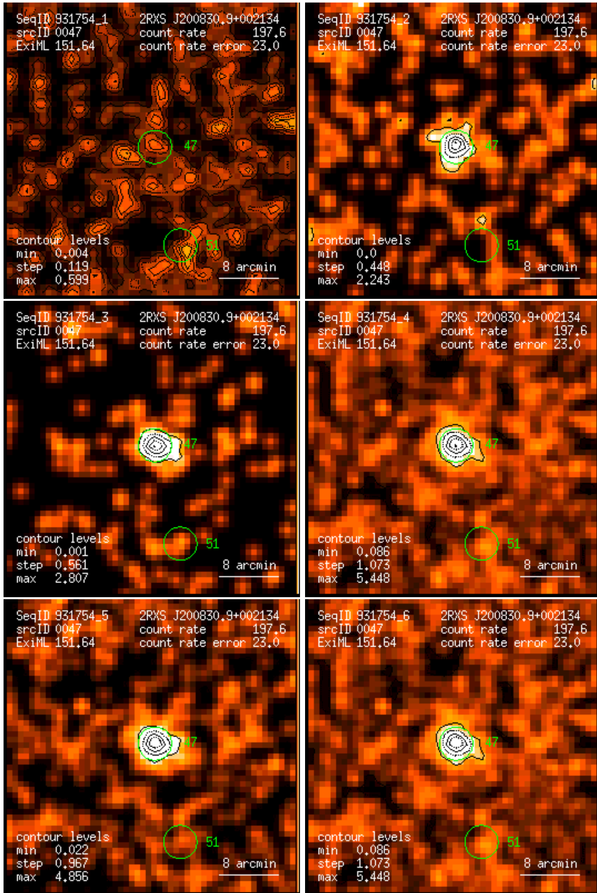
Figure 47: RASS 931754: detection 0047: band rate images, Gaussian filter: (1) PSPC channels 11 – 41, (2) 52 – 90, (3) 91 – 201, (4) 11 – 235, (5) 52 – 201, (6) 11 – 201. Broad band rates in counts/ks. Band rate contour levels in counts/ks/arcmin 2 .
