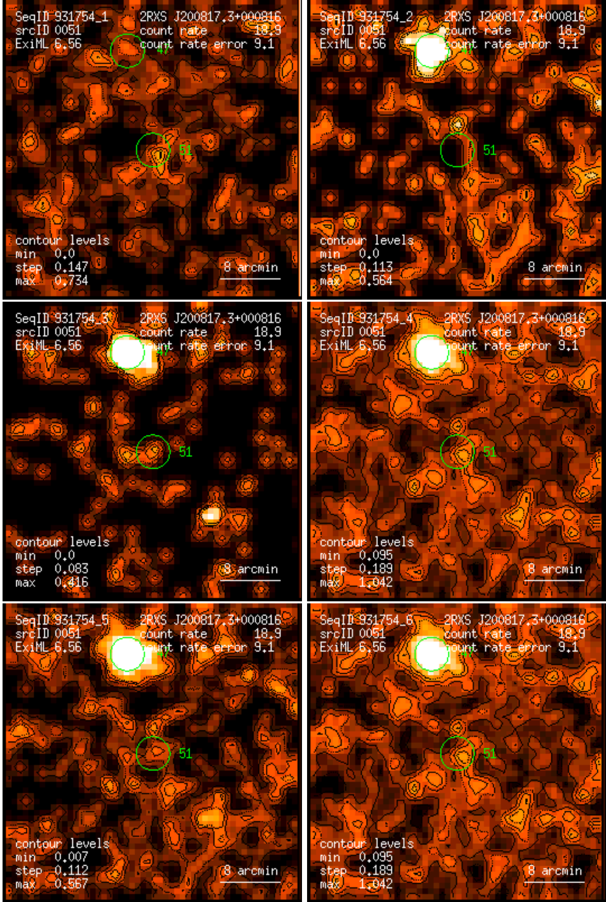
Figure 51: RASS 931754: detection 0051: band rate images, Gaussian filter: (1) PSPC channels 11 – 41, (2) 52 – 90, (3) 91 – 201, (4) 11 – 235, (5) 52 – 201, (6) 11 – 201. Broad band rates in counts/ks. Band rate contour levels in counts/ks/arcmin 2 .
