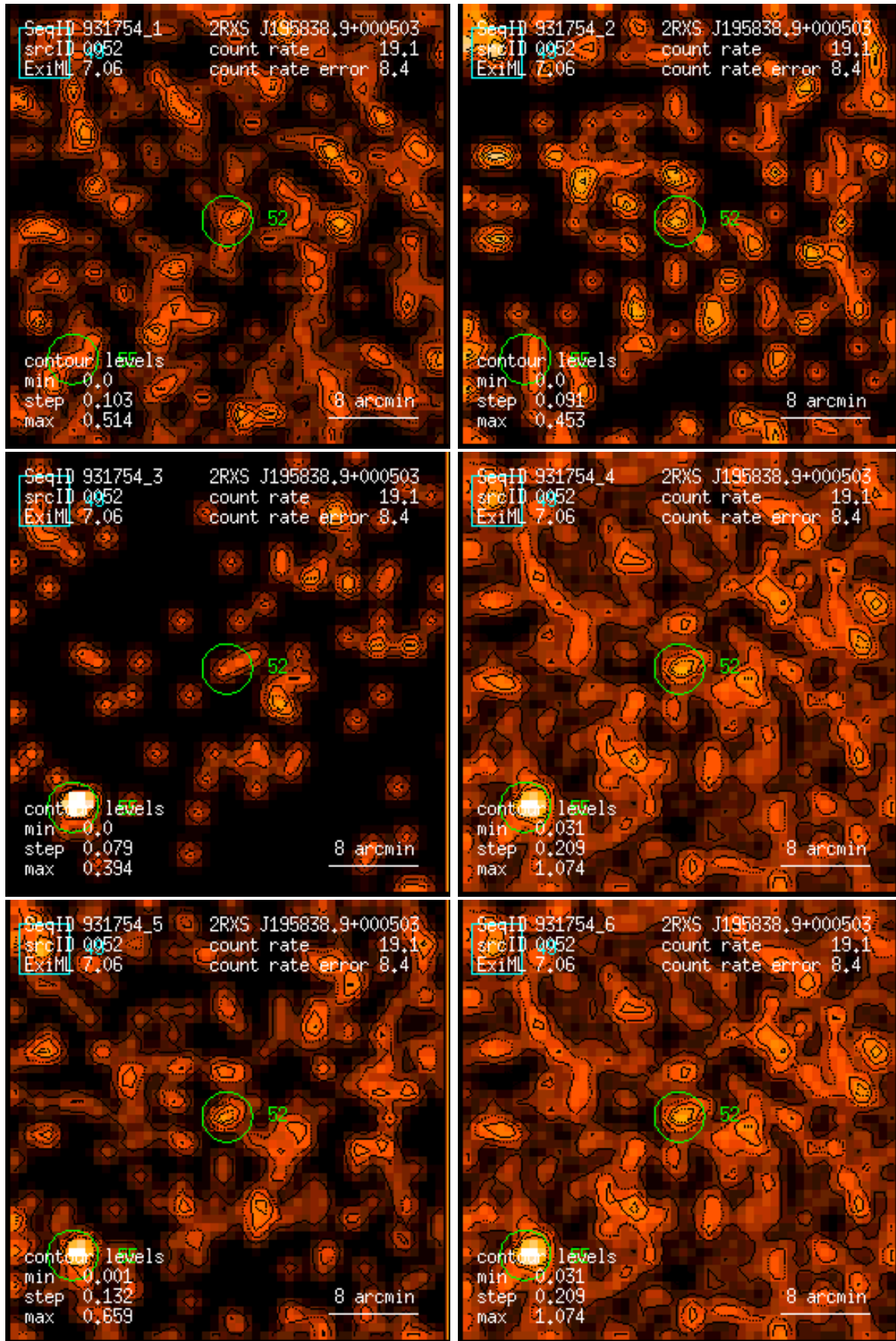
Figure 52: RASS 931754: detection 0052: band rate images, Gaussian filter: (1) PSPC channels 11 – 41, (2) 52 – 90, (3) 91 – 201, (4) 11 – 235, (5) 52 – 201, (6) 11 – 201. Broad band rates in counts/ks. Band rate contour levels in counts/ks/arcmin 2 .
