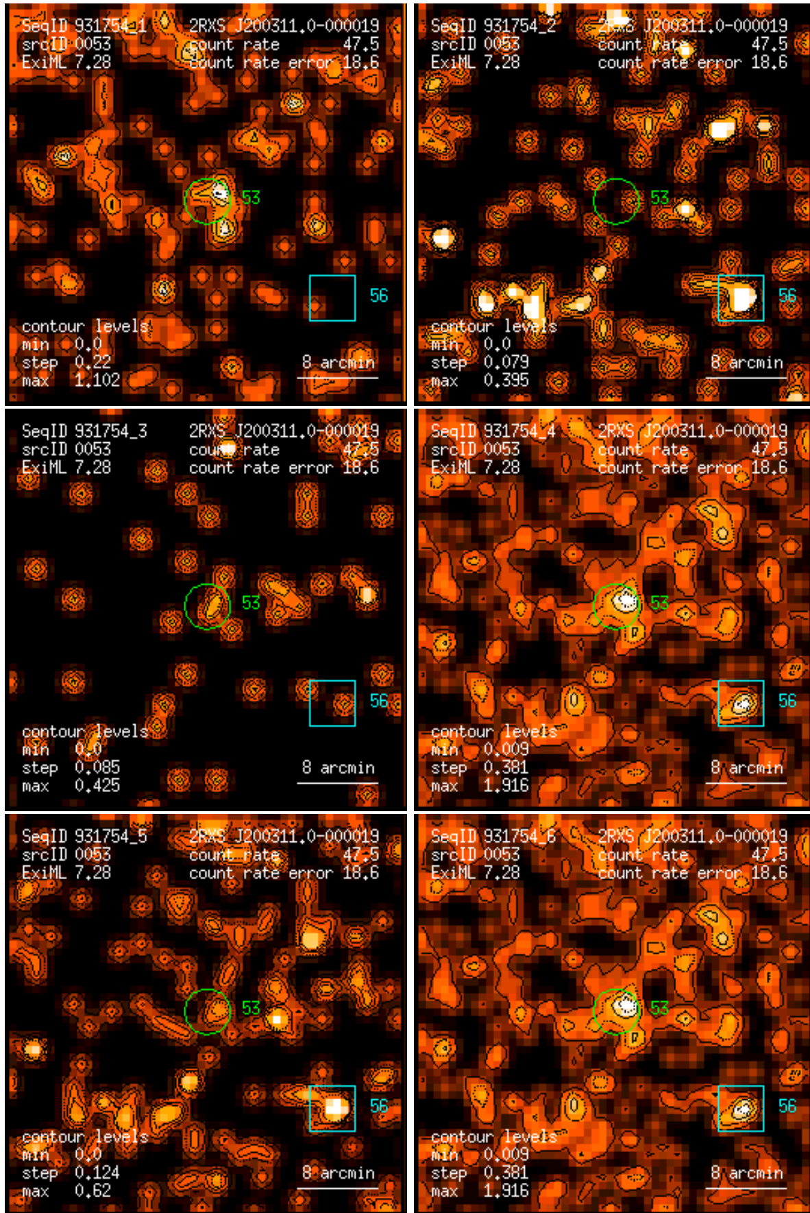
Figure 53: RASS 931754: detection 0053: band rate images, Gaussian filter: (1) PSPC channels 11 – 41, (2) 52 – 90, (3) 91 – 201, (4) 11 – 235, (5) 52 – 201, (6) 11 – 201. Broad band rates in counts/ks. Band rate contour levels in counts/ks/arcmin 2 .
