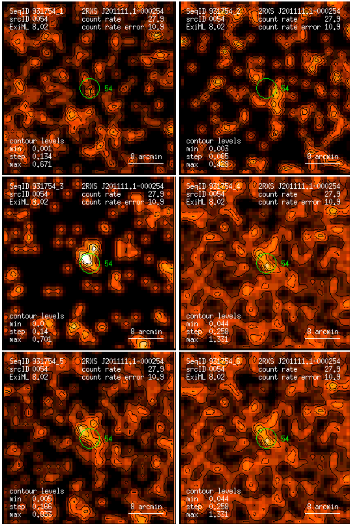
Figure 54: RASS 931754: detection 0054: band rate images, Gaussian filter: (1) PSPC channels 11 – 41, (2) 52 – 90, (3) 91 – 201, (4) 11 – 235, (5) 52 – 201, (6) 11 – 201. Broad band rates in counts/ks. Band rate contour levels in counts/ks/arcmin 2 .
