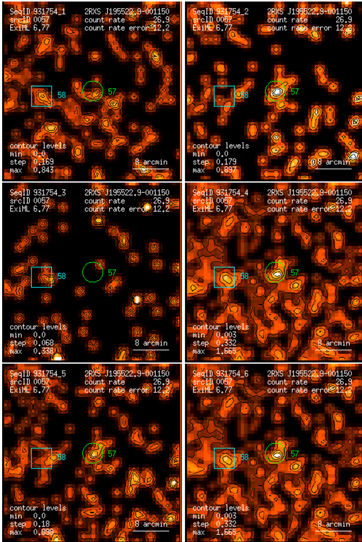
Figure 57: RASS 931754: detection 0057: band rate images, Gaussian filter: (1) PSPC channels 11 – 41, (2) 52 – 90, (3) 91 – 201, (4) 11 – 235, (5) 52 – 201, (6) 11 – 201. Broad band rates in counts/ks. Band rate contour levels in counts/ks/arcmin 2 .
