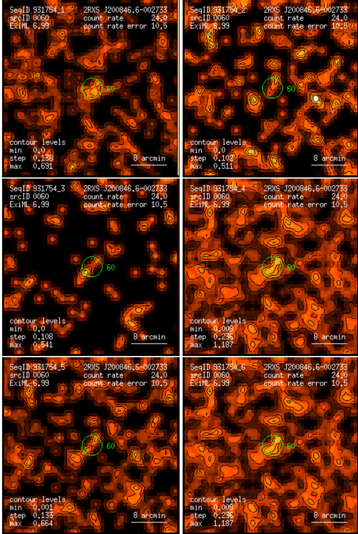
Figure 60: RASS 931754: detection 0060: band rate images, Gaussian filter: (1) PSPC channels 11 – 41, (2) 52 – 90, (3) 91 – 201, (4) 11 – 235, (5) 52 – 201, (6) 11 – 201. Broad band rates in counts/ks. Band rate contour levels in counts/ks/arcmin 2 .
