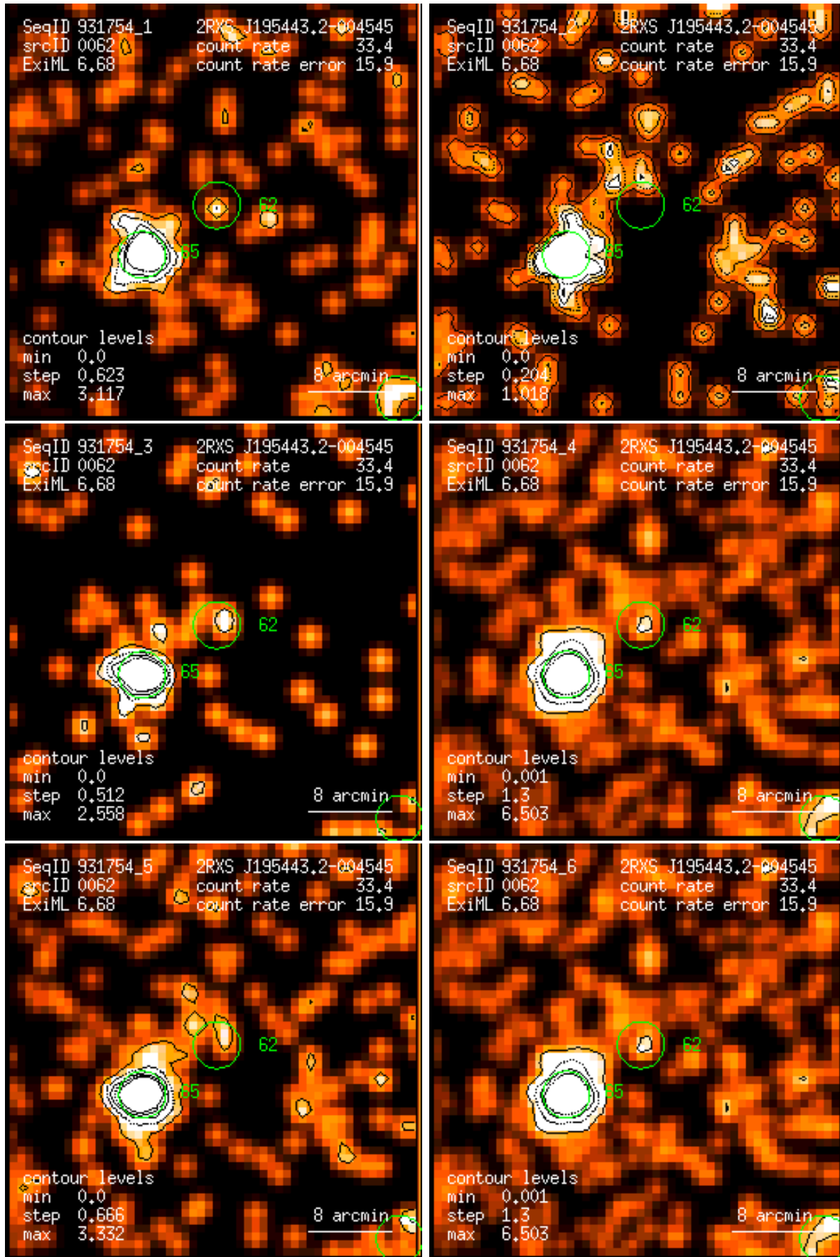
Figure 62: RASS 931754: detection 0062: band rate images, Gaussian filter: (1) PSPC channels 11 – 41, (2) 52 – 90, (3) 91 – 201, (4) 11 – 235, (5) 52 – 201, (6) 11 – 201. Broad band rates in counts/ks. Band rate contour levels in counts/ks/arcmin 2 .
