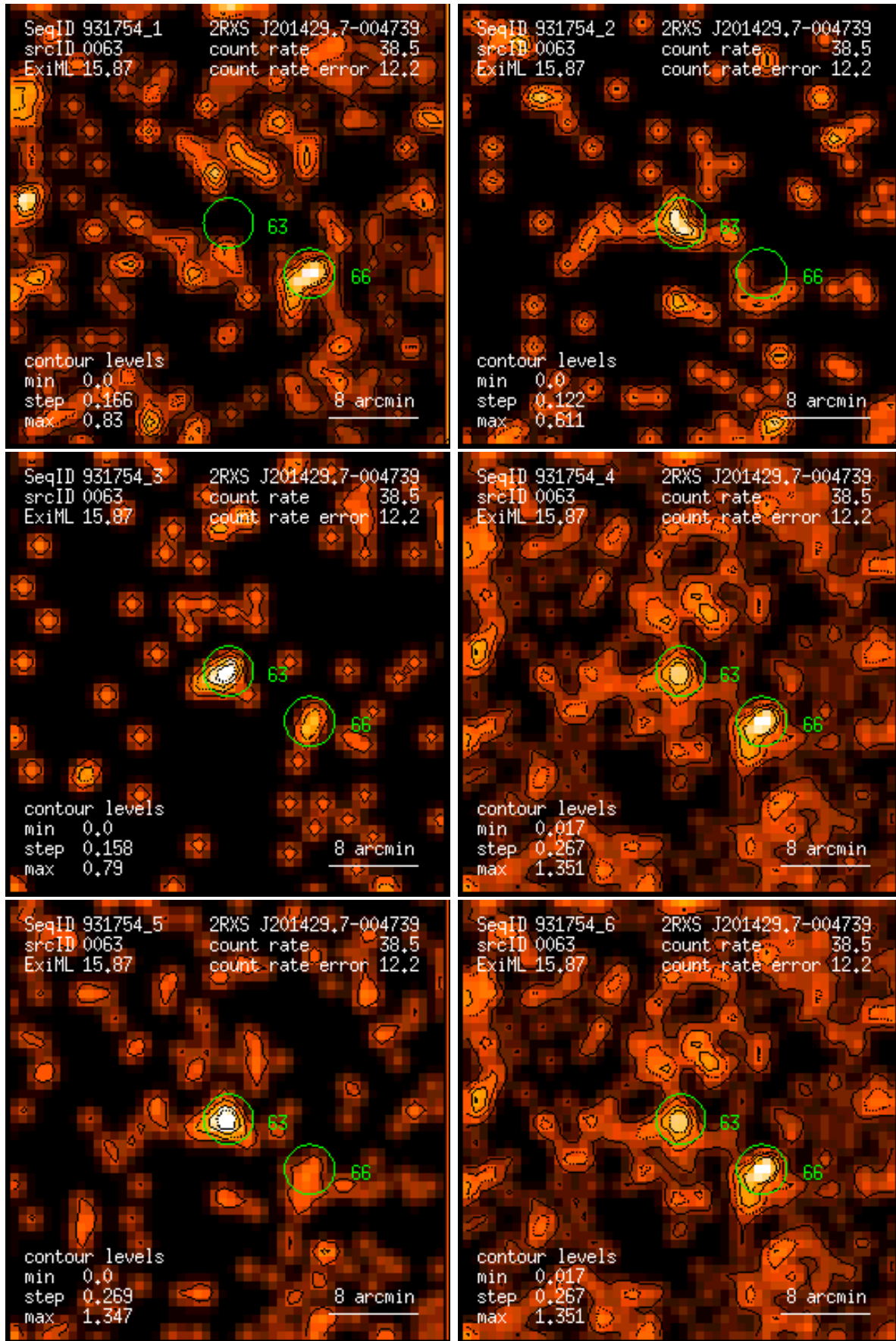
Figure 63: RASS 931754: detection 0063: band rate images, Gaussian filter: (1) PSPC channels 11 – 41, (2) 52 – 90, (3) 91 – 201, (4) 11 – 235, (5) 52 – 201, (6) 11 – 201. Broad band rates in counts/ks. Band rate contour levels in counts/ks/arcmin 2 .
