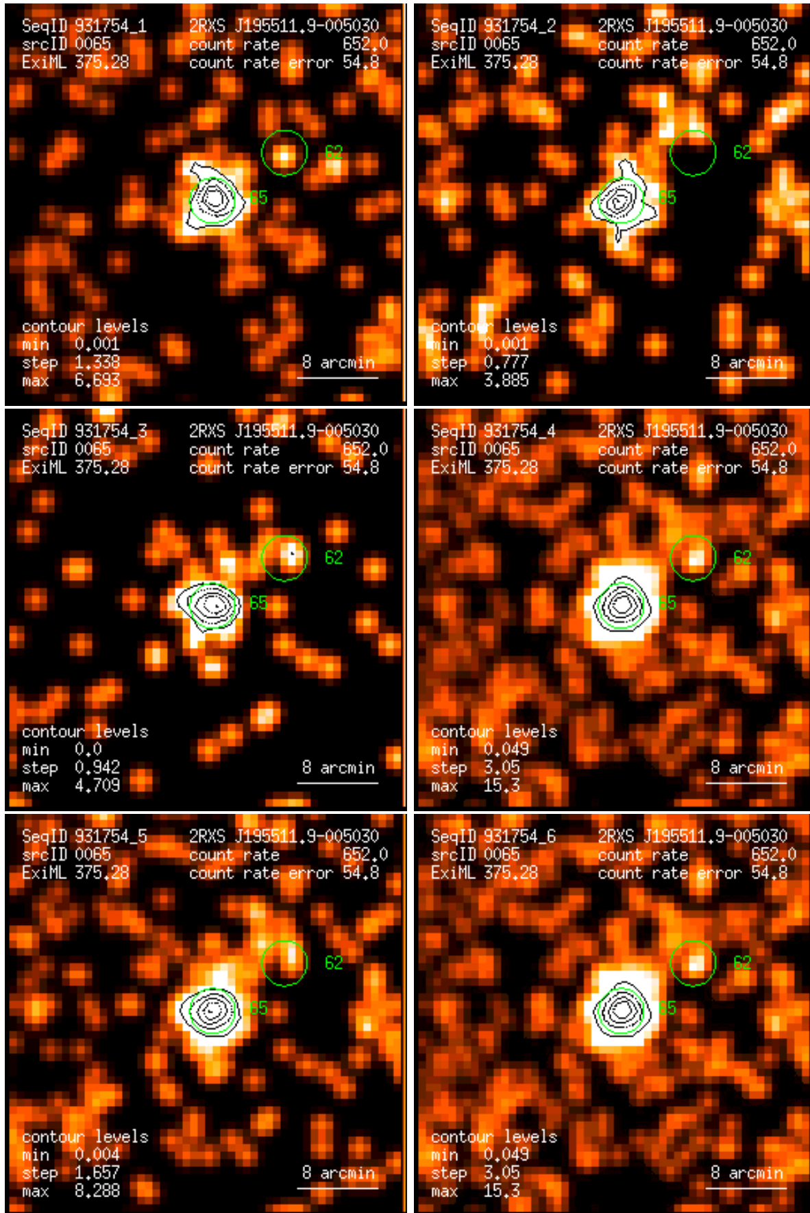
Figure 65: RASS 931754: detection 0065: band rate images, Gaussian filter: (1) PSPC channels 11 – 41, (2) 52 – 90, (3) 91 – 201, (4) 11 – 235, (5) 52 – 201, (6) 11 – 201. Broad band rates in counts/ks. Band rate contour levels in counts/ks/arcmin 2 .
