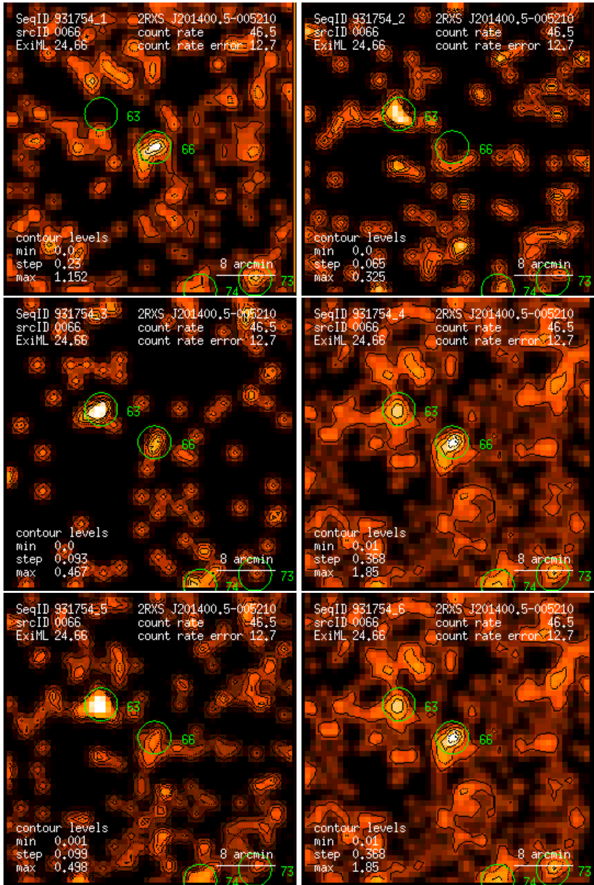
Figure 66: RASS 931754: detection 0066: band rate images, Gaussian filter: (1) PSPC channels 11 – 41, (2) 52 – 90, (3) 91 – 201, (4) 11 – 235, (5) 52 – 201, (6) 11 – 201. Broad band rates in counts/ks. Band rate contour levels in counts/ks/arcmin 2 .
