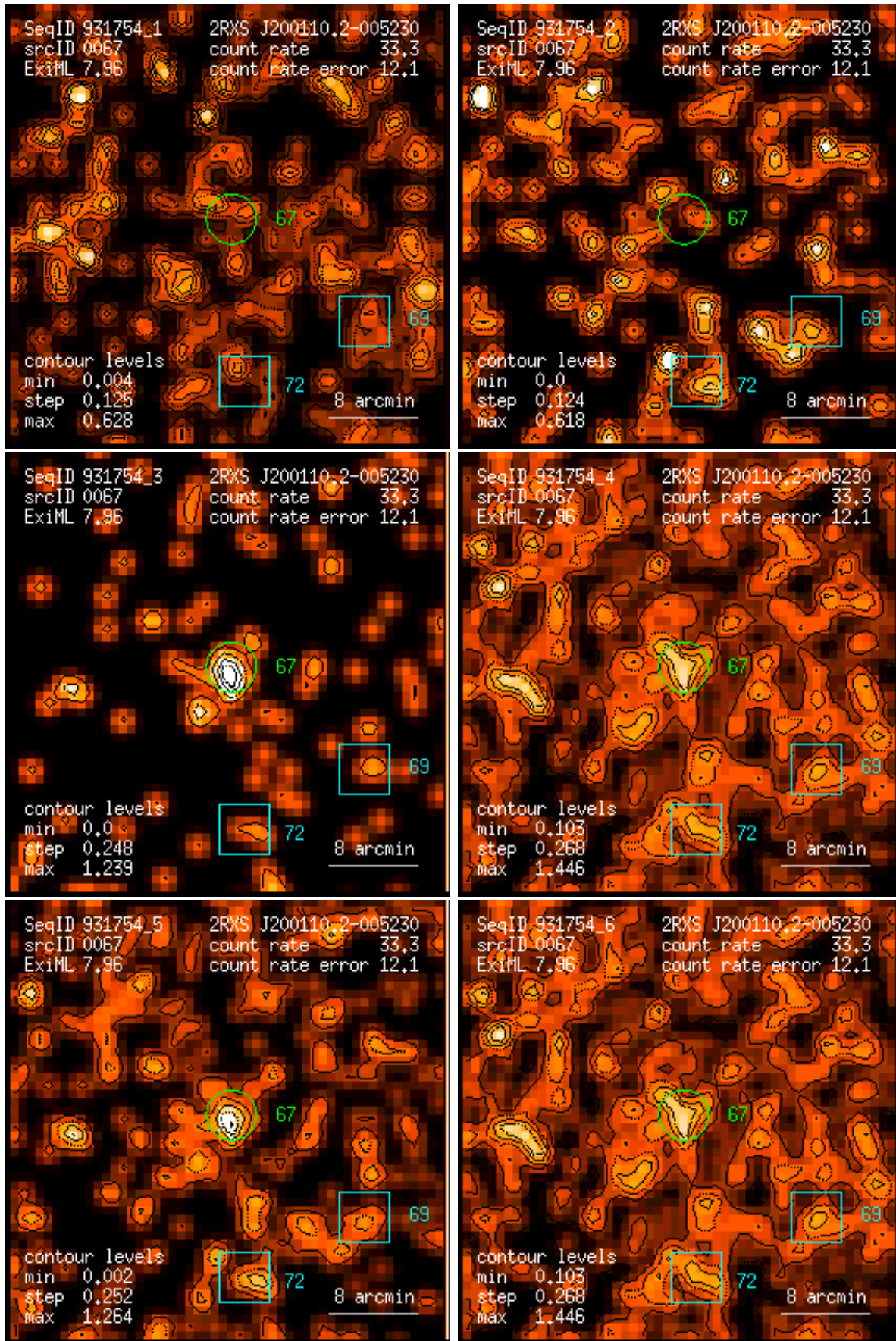
Figure 67: RASS 931754: detection 0067: band rate images, Gaussian filter: (1) PSPC channels 11 – 41, (2) 52 – 90, (3) 91 – 201, (4) 11 – 235, (5) 52 – 201, (6) 11 – 201. Broad band rates in counts/ks. Band rate contour levels in counts/ks/arcmin 2 .
