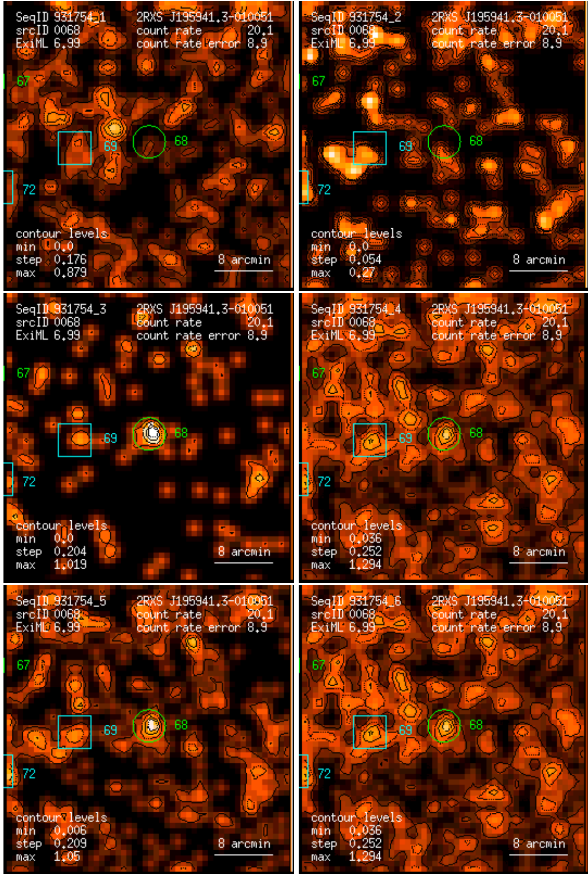
Figure 68: RASS 931754: detection 0068: band rate images, Gaussian filter: (1) PSPC channels 11 – 41, (2) 52 – 90, (3) 91 – 201, (4) 11 – 235, (5) 52 – 201, (6) 11 – 201. Broad band rates in counts/ks. Band rate contour levels in counts/ks/arcmin 2 .
