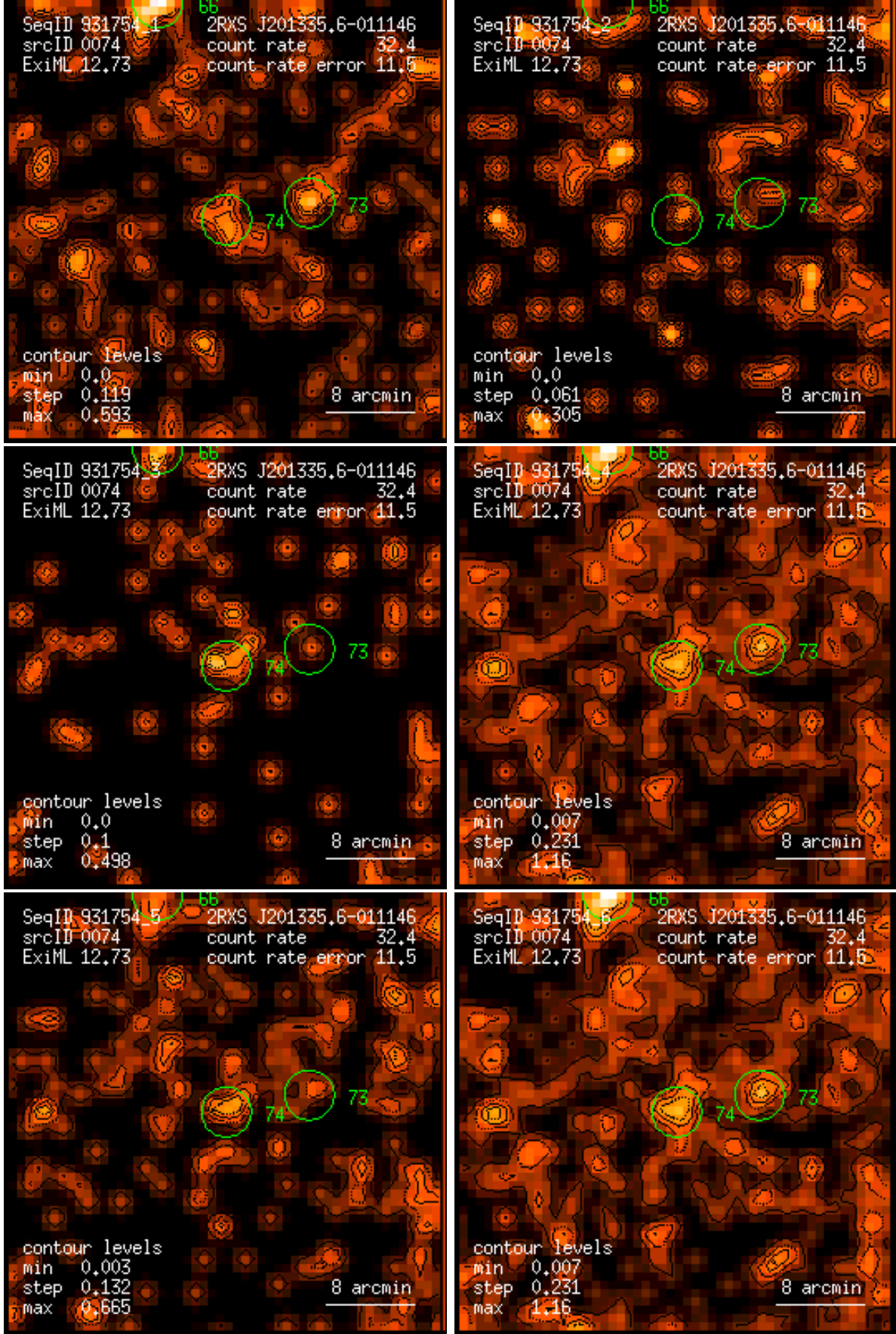
Figure 74: RASS 931754: detection 0074: band rate images, Gaussian filter: (1) PSPC channels 11 – 41, (2) 52 – 90, (3) 91 – 201, (4) 11 – 235, (5) 52 – 201, (6) 11 – 201. Broad band rates in counts/ks. Band rate contour levels in counts/ks/arcmin 2 .
