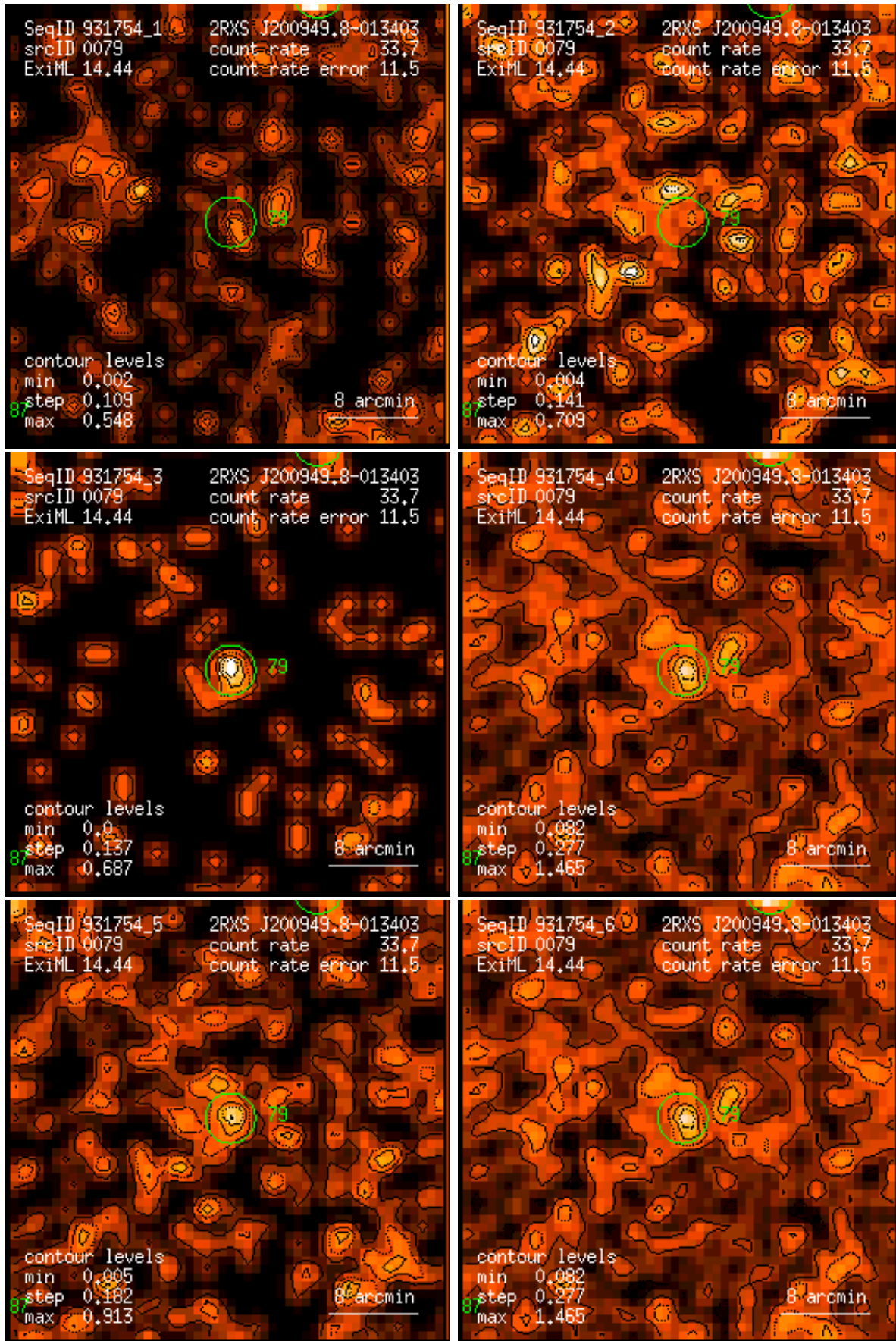
Figure 79: RASS 931754: detection 0079: band rate images, Gaussian filter: (1) PSPC channels 11 – 41, (2) 52 – 90, (3) 91 – 201, (4) 11 – 235, (5) 52 – 201, (6) 11 – 201. Broad band rates in counts/ks. Band rate contour levels in counts/ks/arcmin 2 .
