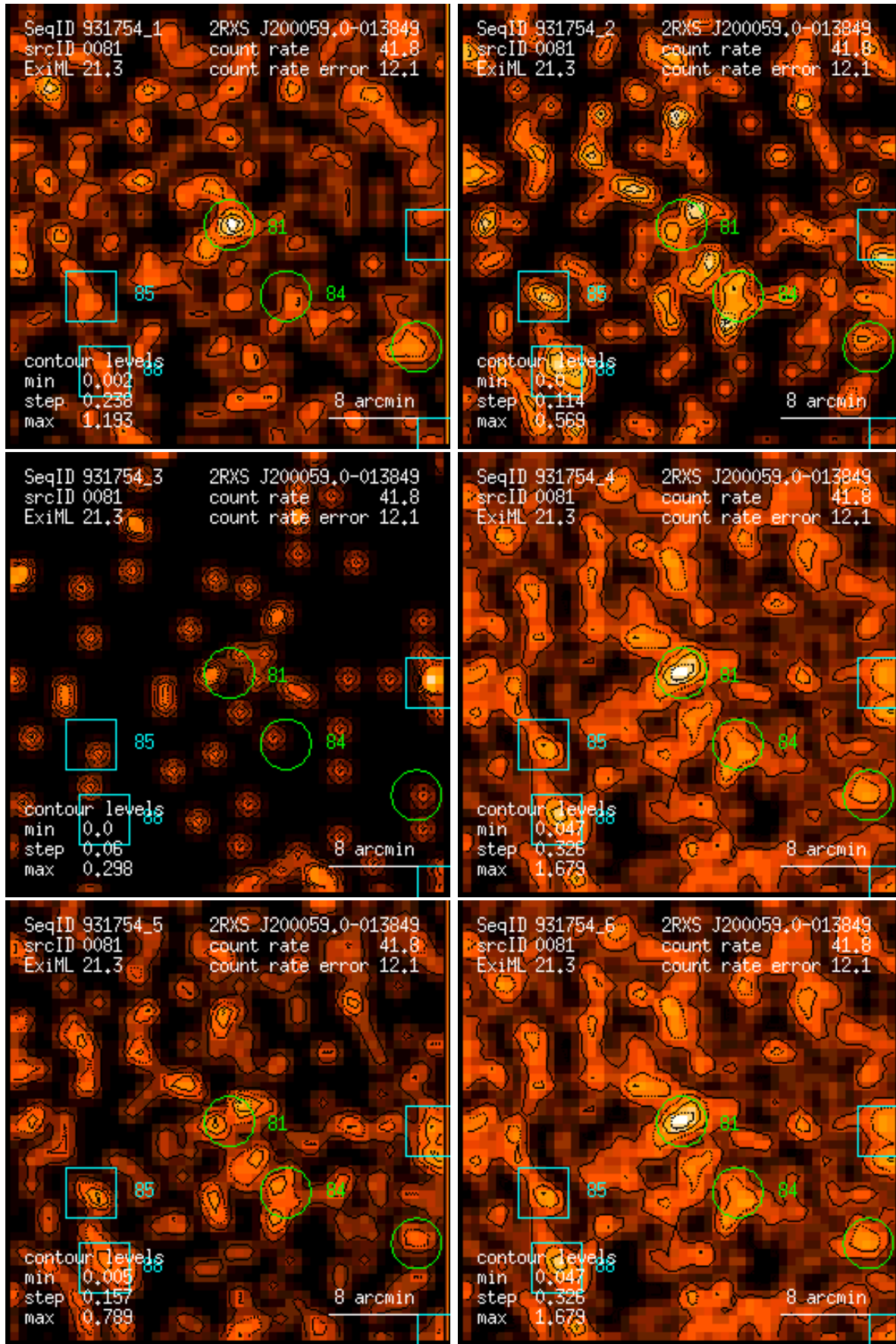
Figure 81: RASS 931754: detection 0081: band rate images, Gaussian filter: (1) PSPC channels 11 – 41, (2) 52 – 90, (3) 91 – 201, (4) 11 – 235, (5) 52 – 201, (6) 11 – 201. Broad band rates in counts/ks. Band rate contour levels in counts/ks/arcmin 2 .
