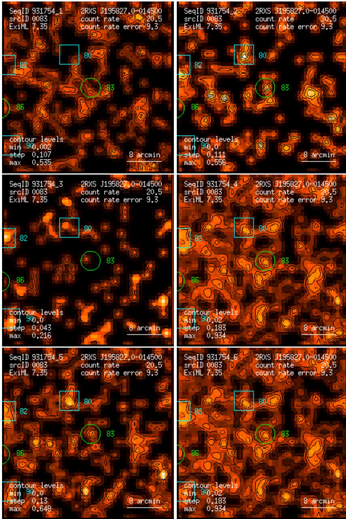
Figure 83: RASS 931754: detection 0083: band rate images, Gaussian filter: (1) PSPC channels 11 – 41, (2) 52 – 90, (3) 91 – 201, (4) 11 – 235, (5) 52 – 201, (6) 11 – 201. Broad band rates in counts/ks. Band rate contour levels in counts/ks/arcmin 2 .
