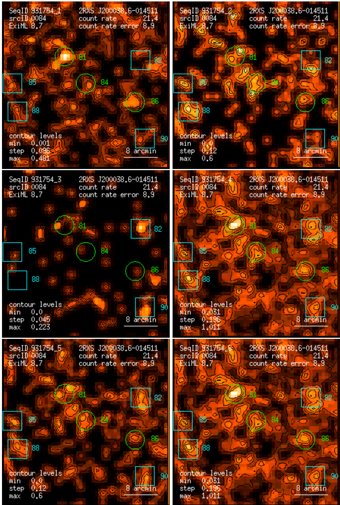
Figure 84: RASS 931754: detection 0084: band rate images, Gaussian filter: (1) PSPC channels 11 – 41, (2) 52 – 90, (3) 91 – 201, (4) 11 – 235, (5) 52 – 201, (6) 11 – 201. Broad band rates in counts/ks. Band rate contour levels in counts/ks/arcmin 2 .
