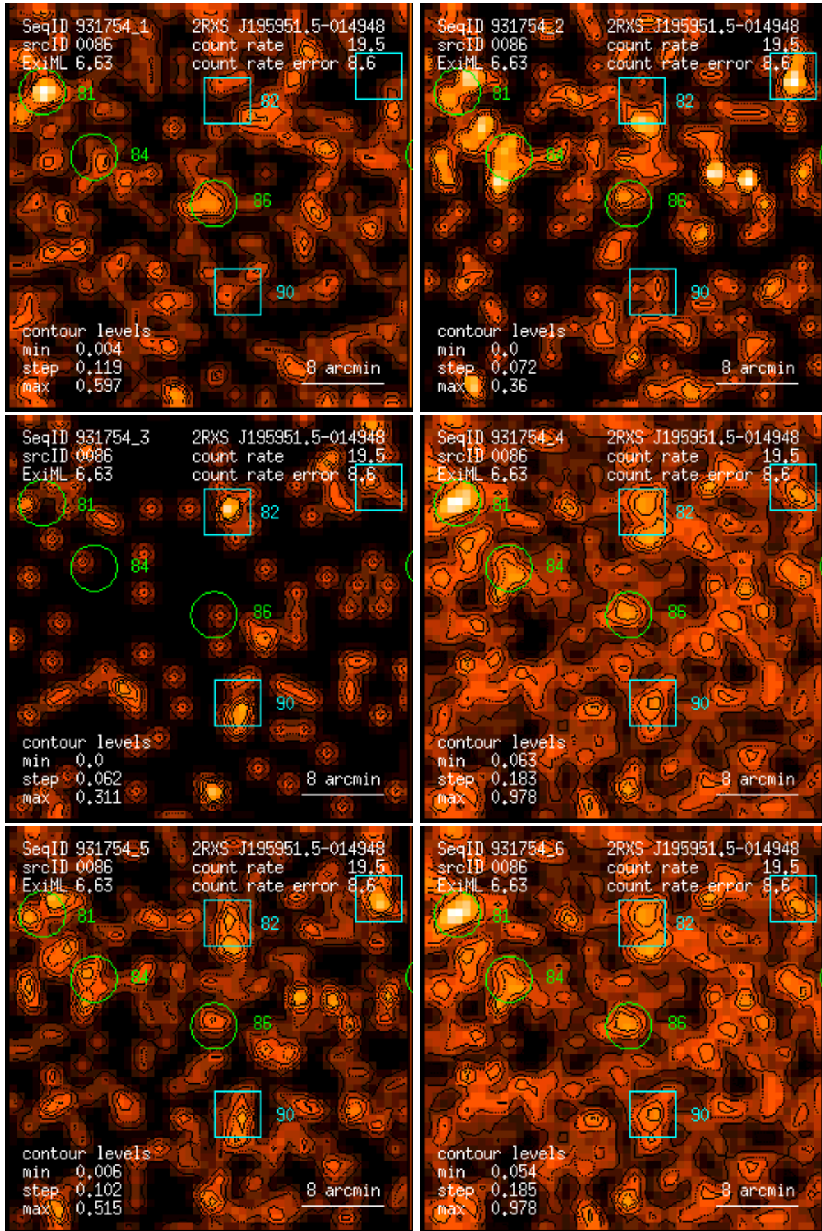
Figure 86: RASS 931754: detection 0086: band rate images, Gaussian filter: (1) PSPC channels 11 – 41, (2) 52 – 90, (3) 91 – 201, (4) 11 – 235, (5) 52 – 201, (6) 11 – 201. Broad band rates in counts/ks. Band rate contour levels in counts/ks/arcmin 2 .
