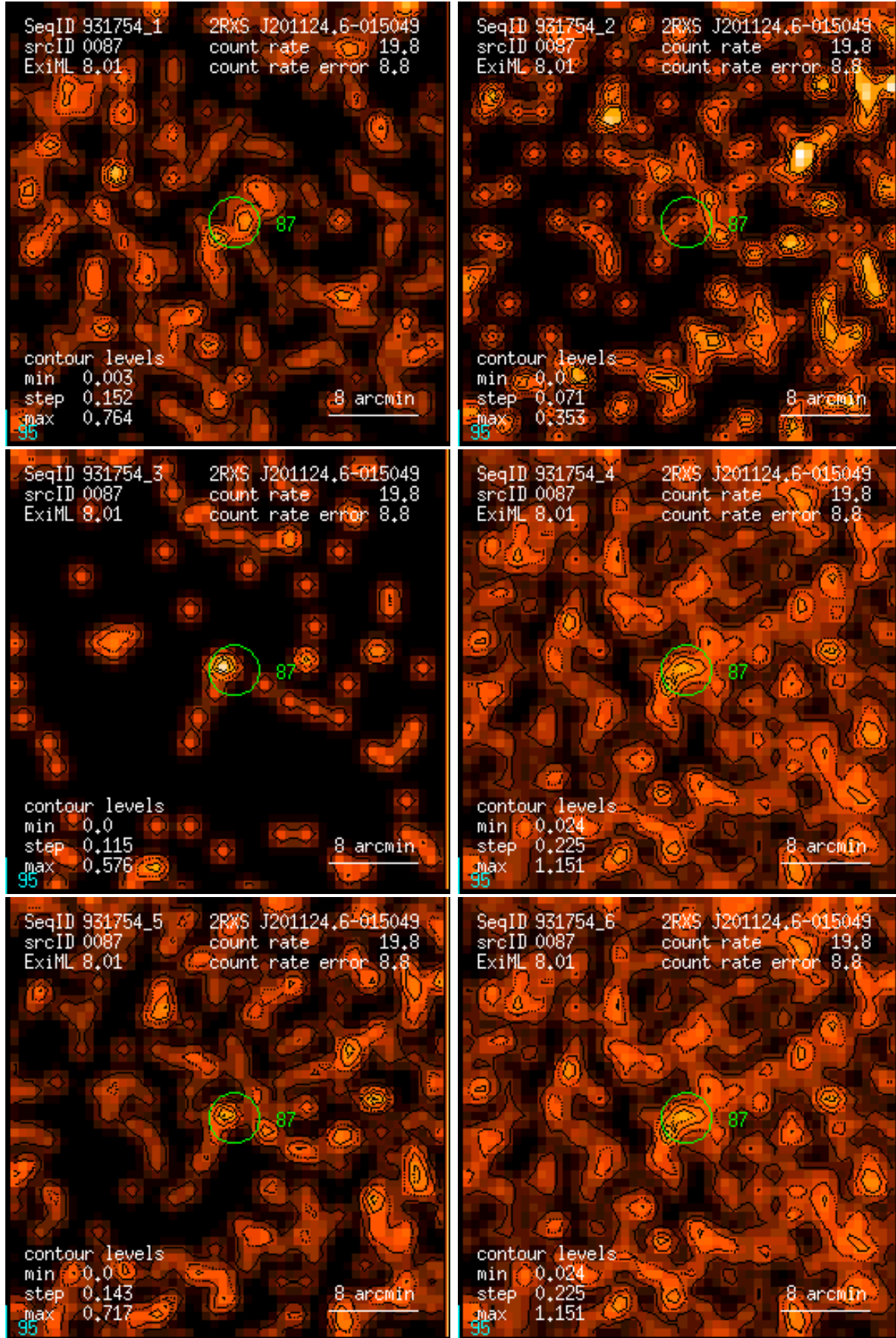
Figure 87: RASS 931754: detection 0087: band rate images, Gaussian filter: (1) PSPC channels 11 – 41, (2) 52 – 90, (3) 91 – 201, (4) 11 – 235, (5) 52 – 201, (6) 11 – 201. Broad band rates in counts/ks. Band rate contour levels in counts/ks/arcmin 2 .
