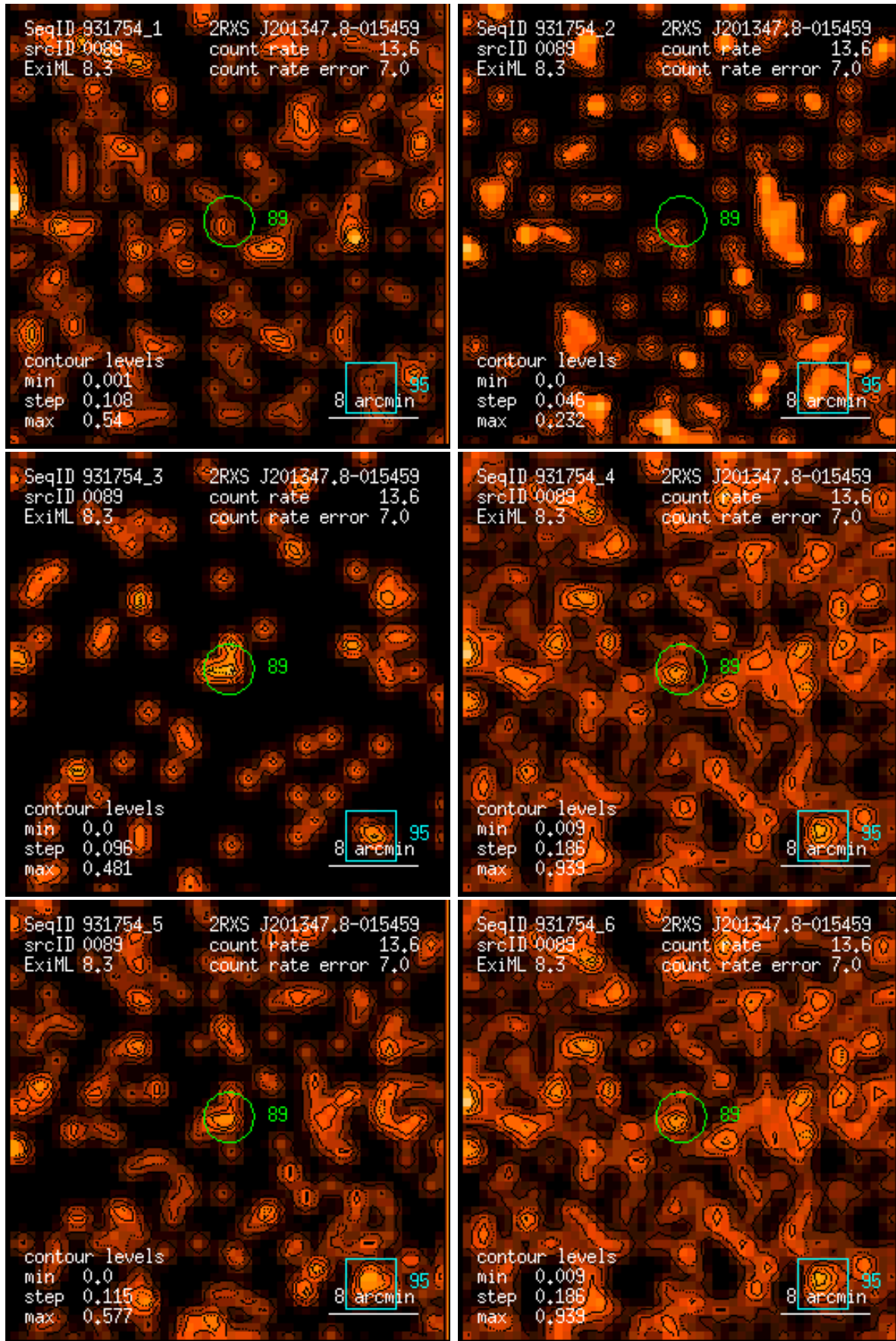
Figure 89: RASS 931754: detection 0089: band rate images, Gaussian filter: (1) PSPC channels 11 – 41, (2) 52 – 90, (3) 91 – 201, (4) 11 – 235, (5) 52 – 201, (6) 11 – 201. Broad band rates in counts/ks. Band rate contour levels in counts/ks/arcmin 2 .
