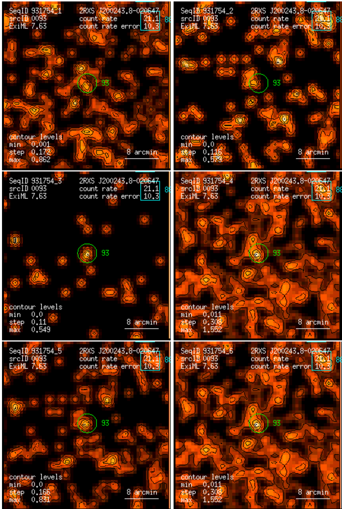
Figure 93: RASS 931754: detection 0093: band rate images, Gaussian filter: (1) PSPC channels 11 – 41, (2) 52 – 90, (3) 91 – 201, (4) 11 – 235, (5) 52 – 201, (6) 11 – 201. Broad band rates in counts/ks. Band rate contour levels in counts/ks/arcmin 2 .
