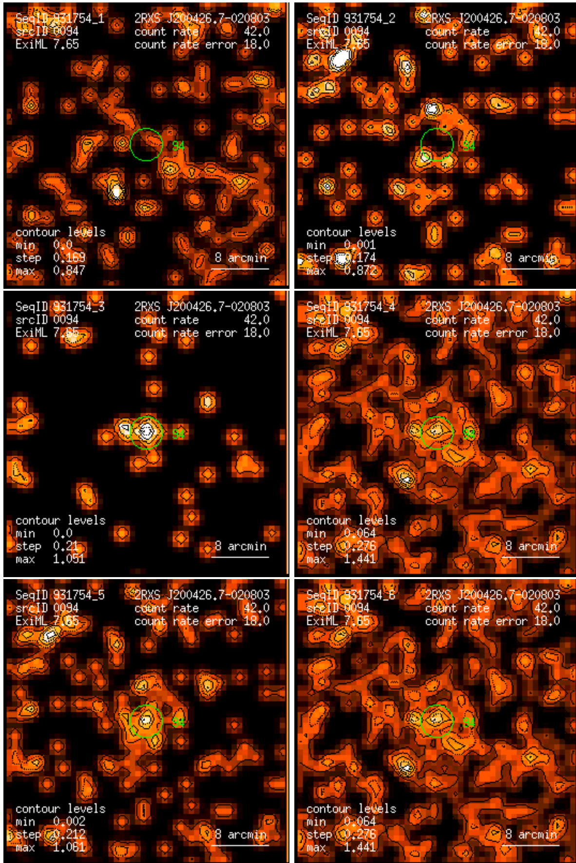
Figure 94: RASS 931754: detection 0094: band rate images, Gaussian filter: (1) PSPC channels 11 – 41, (2) 52 – 90, (3) 91 – 201, (4) 11 – 235, (5) 52 – 201, (6) 11 – 201. Broad band rates in counts/ks. Band rate contour levels in counts/ks/arcmin 2 .
