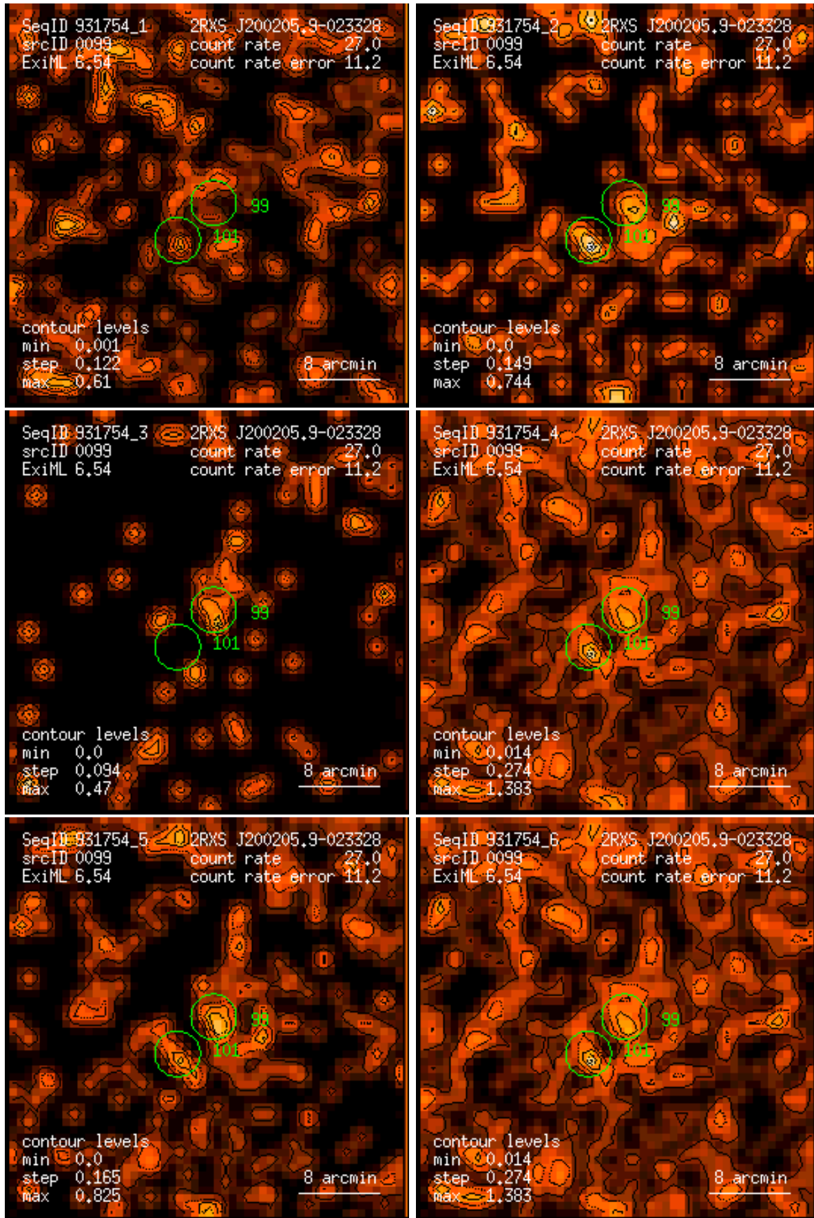
Figure 99: RASS 931754: detection 0099: band rate images, Gaussian filter: (1) PSPC channels 11 – 41, (2) 52 – 90, (3) 91 – 201, (4) 11 – 235, (5) 52 – 201, (6) 11 – 201. Broad band rates in counts/ks. Band rate contour levels in counts/ks/arcmin 2 .
