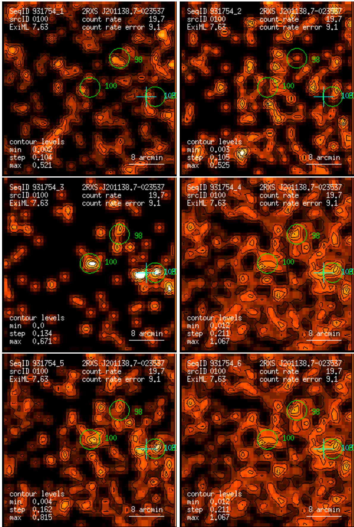
Figure 100: RASS 931754: detection 0100: band rate images, Gaussian filter: (1) PSPC channels 11 – 41, (2) 52 – 90, (3) 91 – 201, (4) 11 – 235, (5) 52 – 201, (6) 11 – 201. Broad band rates in counts/ks. Band rate contour levels in counts/ks/arcmin 2 .
