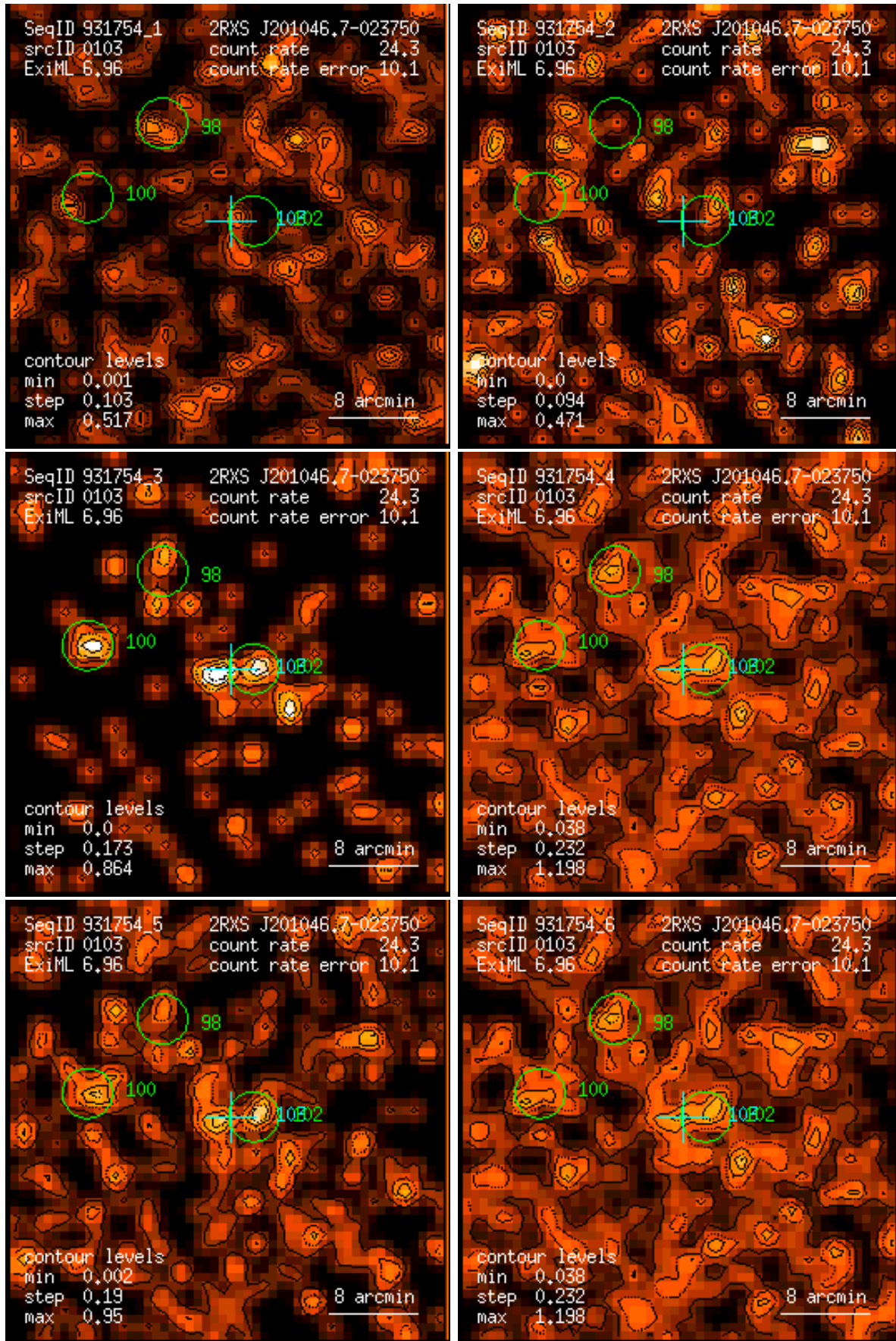
Figure 103: RASS 931754: detection 0103: band rate images, Gaussian filter: (1) PSPC channels 11 – 41, (2) 52 – 90, (3) 91 – 201, (4) 11 – 235, (5) 52 – 201, (6) 11 – 201. Broad band rates in counts/ks. Band rate contour levels in counts/ks/arcmin 2 .
