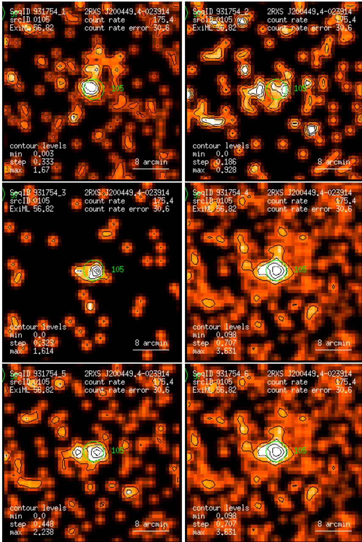
Figure 105: RASS 931754: detection 0105: band rate images, Gaussian filter: (1) PSPC channels 11 – 41, (2) 52 – 90, (3) 91 – 201, (4) 11 – 235, (5) 52 – 201, (6) 11 – 201. Broad band rates in counts/ks. Band rate contour levels in counts/ks/arcmin 2 .
