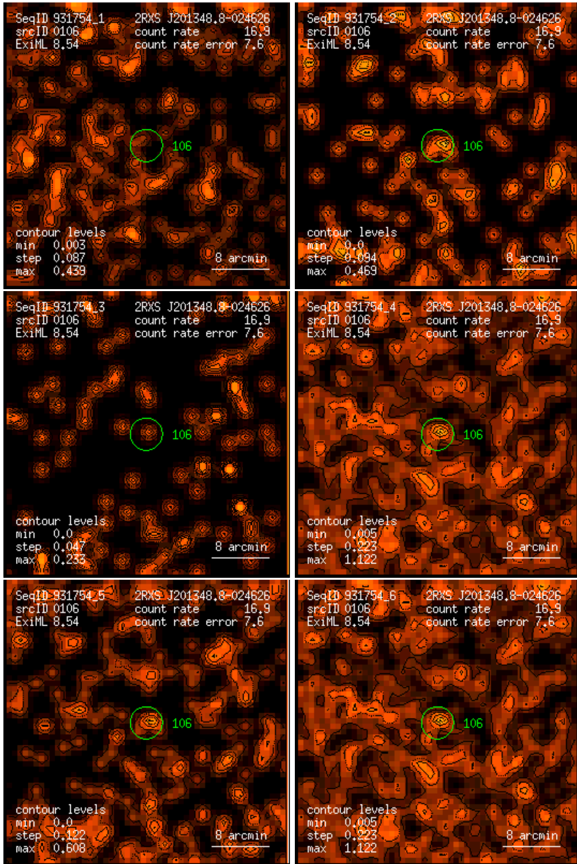
Figure 106: RASS 931754: detection 0106: band rate images, Gaussian filter: (1) PSPC channels 11 – 41, (2) 52 – 90, (3) 91 – 201, (4) 11 – 235, (5) 52 – 201, (6) 11 – 201. Broad band rates in counts/ks. Band rate contour levels in counts/ks/arcmin 2 .
