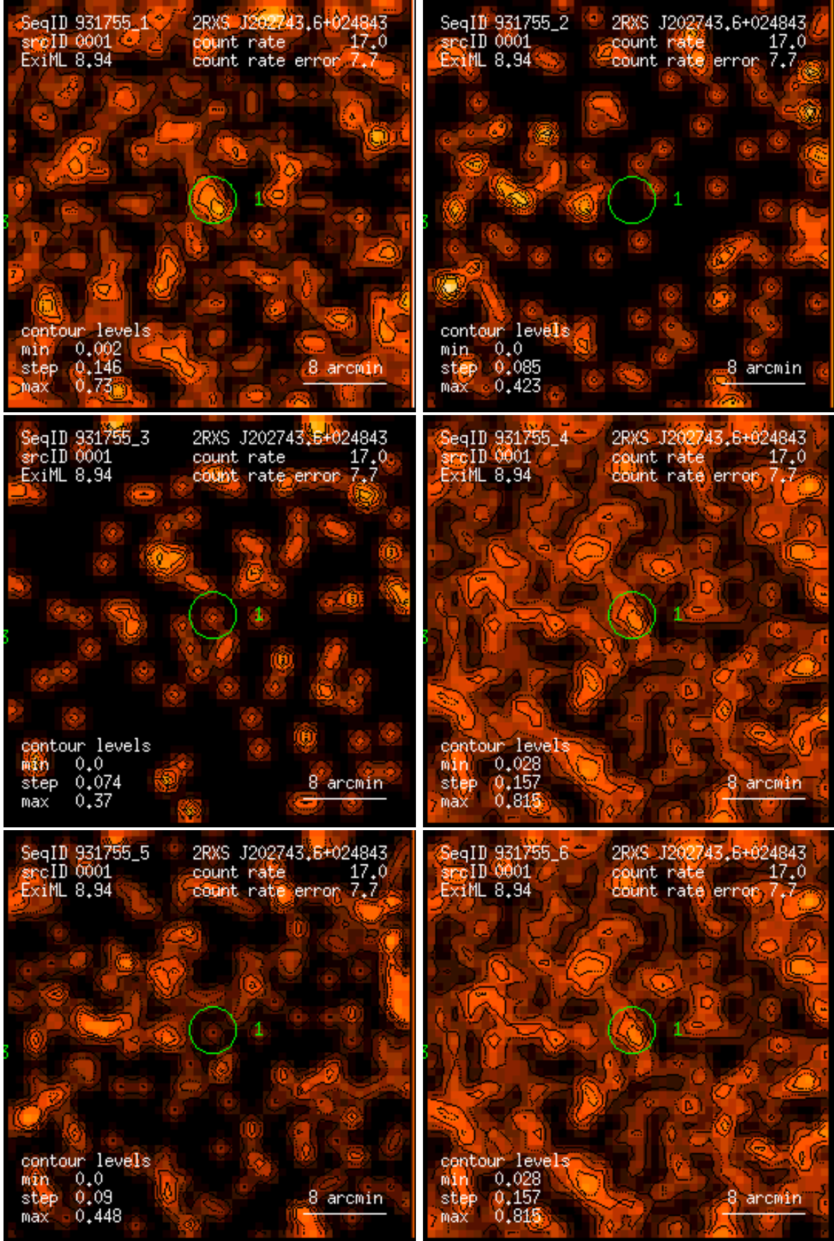
Figure 1: RASS 931755: detection 0001: band rate images, Gaussian filter: (1) PSPC channels 11 – 41, (2) 52 – 90, (3) 91 – 201, (4) 11 – 235, (5) 52 – 201, (6) 11 – 201. Broad band rates in counts/ks. Band rate contour levels in counts/ks/arcmin 2 .
