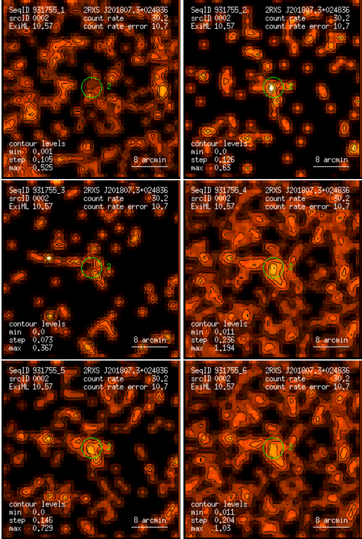
Figure 2: RASS 931755: detection 0002: band rate images, Gaussian filter: (1) PSPC channels 11 – 41, (2) 52 – 90, (3) 91 – 201, (4) 11 – 235, (5) 52 – 201, (6) 11 – 201. Broad band rates in counts/ks. Band rate contour levels in counts/ks/arcmin 2 .
