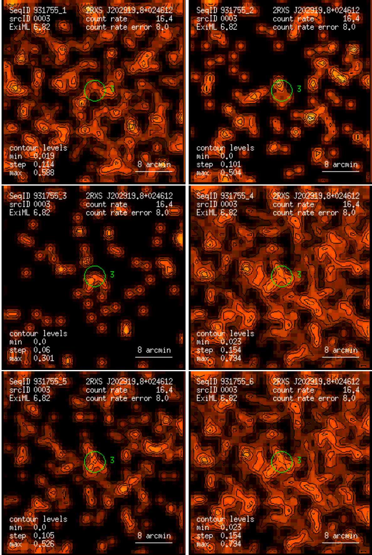
Figure 3: RASS 931755: detection 0003: band rate images, Gaussian filter: (1) PSPC channels 11 – 41, (2) 52 – 90, (3) 91 – 201, (4) 11 – 235, (5) 52 – 201, (6) 11 – 201. Broad band rates in counts/ks. Band rate contour levels in counts/ks/arcmin 2 .
