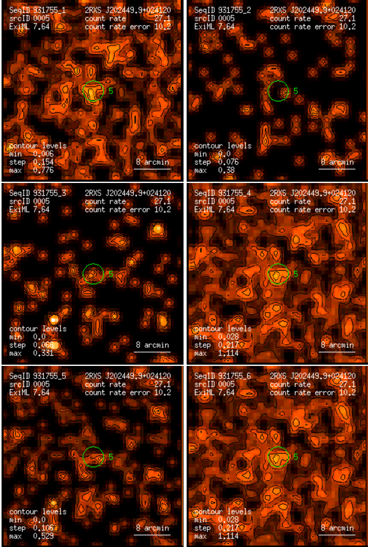
Figure 5: RASS 931755: detection 0005: band rate images, Gaussian filter: (1) PSPC channels 11 – 41, (2) 52 – 90, (3) 91 – 201, (4) 11 – 235, (5) 52 – 201, (6) 11 – 201. Broad band rates in counts/ks. Band rate contour levels in counts/ks/arcmin 2 .
