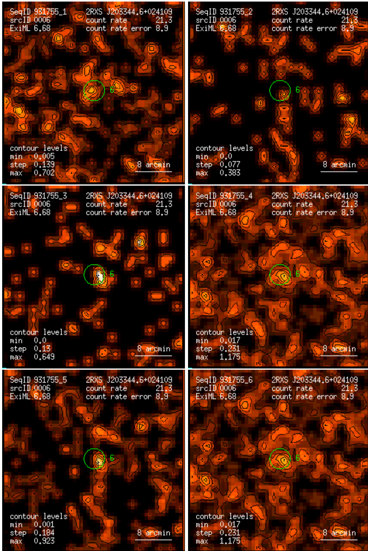
Figure 6: RASS 931755: detection 0006: band rate images, Gaussian filter: (1) PSPC channels 11 – 41, (2) 52 – 90, (3) 91 – 201, (4) 11 – 235, (5) 52 – 201, (6) 11 – 201. Broad band rates in counts/ks. Band rate contour levels in counts/ks/arcmin 2 .
