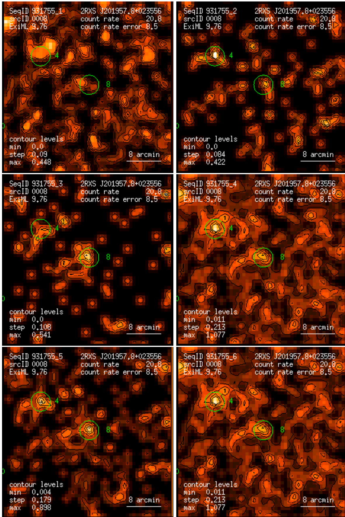
Figure 8: RASS 931755: detection 0008: band rate images, Gaussian filter: (1) PSPC channels 11 – 41, (2) 52 – 90, (3) 91 – 201, (4) 11 – 235, (5) 52 – 201, (6) 11 – 201. Broad band rates in counts/ks. Band rate contour levels in counts/ks/arcmin 2 .
