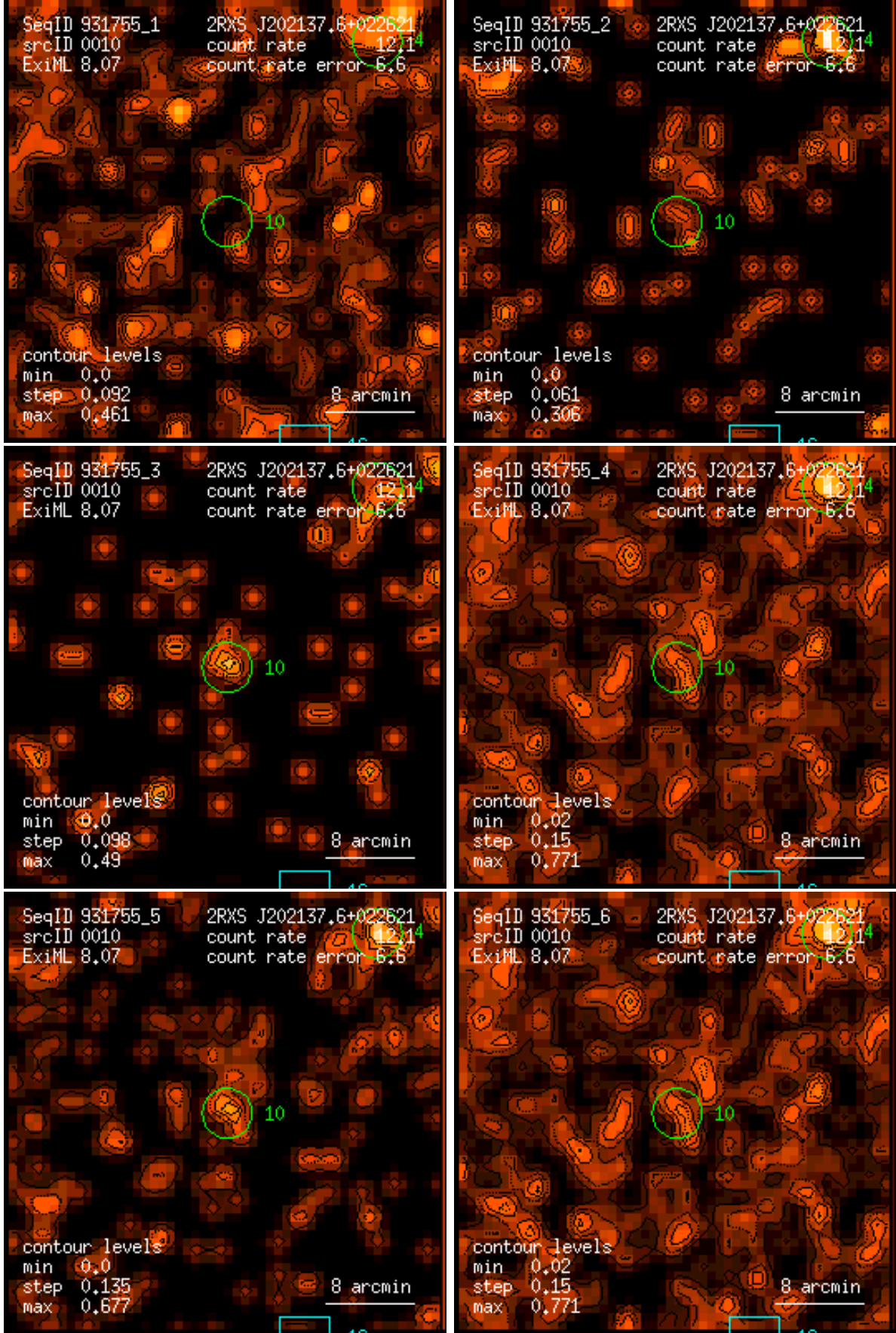
Figure 10: RASS 931755: detection 0010: band rate images, Gaussian filter: (1) PSPC channels 11 – 41, (2) 52 – 90, (3) 91 – 201, (4) 11 – 235, (5) 52 – 201, (6) 11 – 201. Broad band rates in counts/ks. Band rate contour levels in counts/ks/arcmin 2 .
