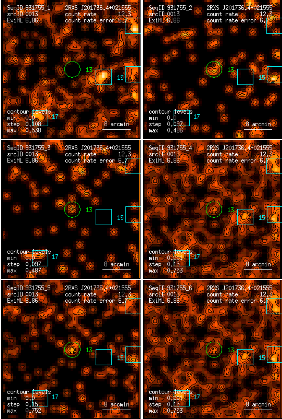
Figure 13: RASS 931755: detection 0013: band rate images, Gaussian filter: (1) PSPC channels 11 – 41, (2) 52 – 90, (3) 91 – 201, (4) 11 – 235, (5) 52 – 201, (6) 11 – 201. Broad band rates in counts/ks. Band rate contour levels in counts/ks/arcmin 2 .
