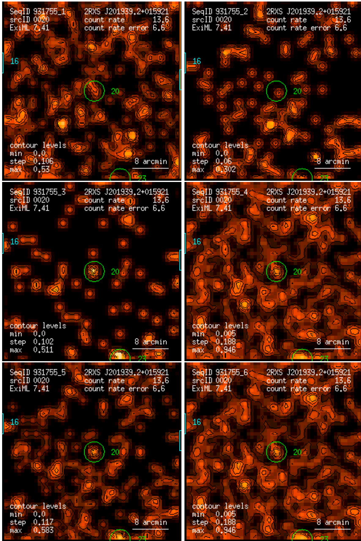
Figure 20: RASS 931755: detection 0020: band rate images, Gaussian filter: (1) PSPC channels 11 – 41, (2) 52 – 90, (3) 91 – 201, (4) 11 – 235, (5) 52 – 201, (6) 11 – 201. Broad band rates in counts/ks. Band rate contour levels in counts/ks/arcmin 2 .
