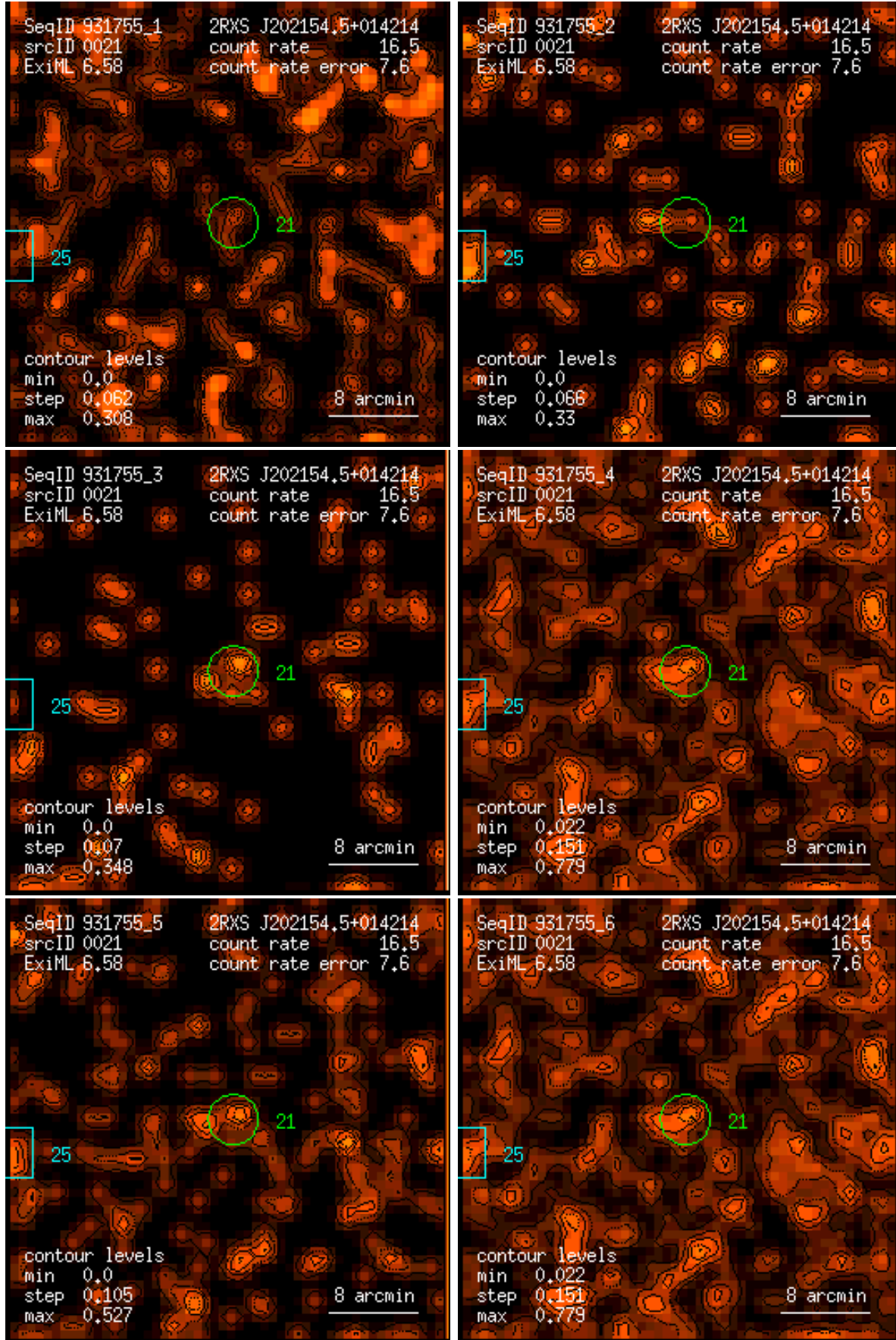
Figure 21: RASS 931755: detection 0021: band rate images, Gaussian filter: (1) PSPC channels 11 – 41, (2) 52 – 90, (3) 91 – 201, (4) 11 – 235, (5) 52 – 201, (6) 11 – 201. Broad band rates in counts/ks. Band rate contour levels in counts/ks/arcmin 2 .
