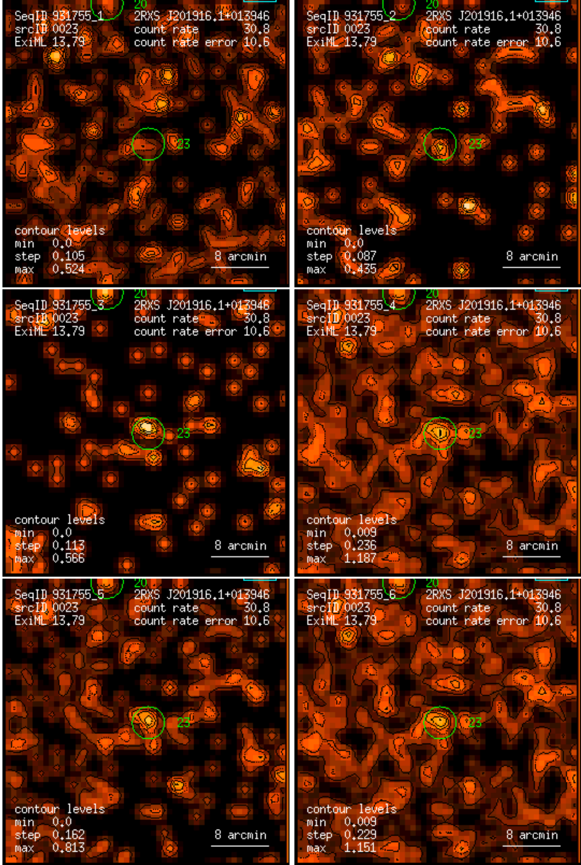
Figure 23: RASS 931755: detection 0023: band rate images, Gaussian filter: (1) PSPC channels 11 – 41, (2) 52 – 90, (3) 91 – 201, (4) 11 – 235, (5) 52 – 201, (6) 11 – 201. Broad band rates in counts/ks. Band rate contour levels in counts/ks/arcmin 2 .
