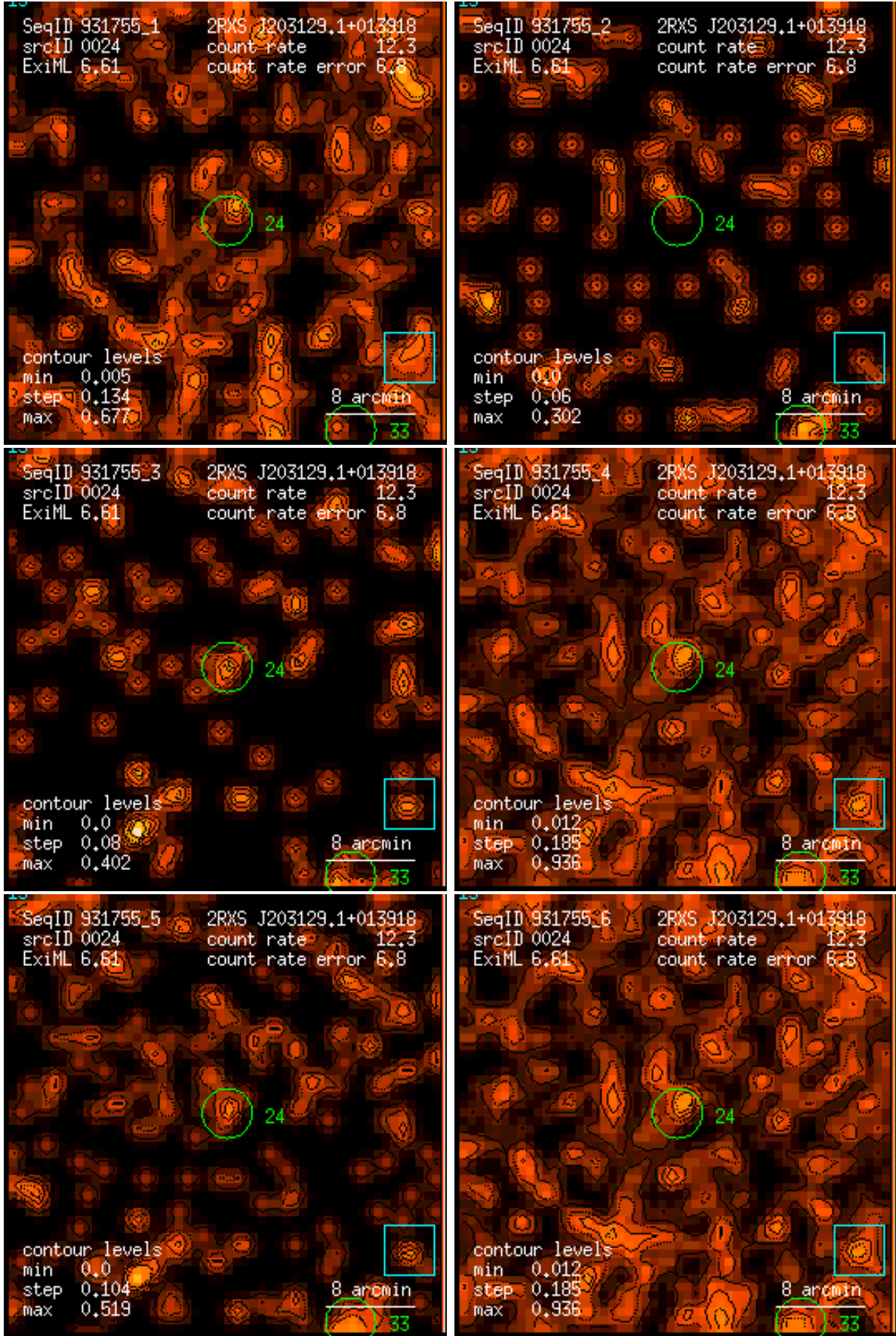
Figure 24: RASS 931755: detection 0024: band rate images, Gaussian filter: (1) PSPC channels 11 – 41, (2) 52 – 90, (3) 91 – 201, (4) 11 – 235, (5) 52 – 201, (6) 11 – 201. Broad band rates in counts/ks. Band rate contour levels in counts/ks/arcmin 2 .
