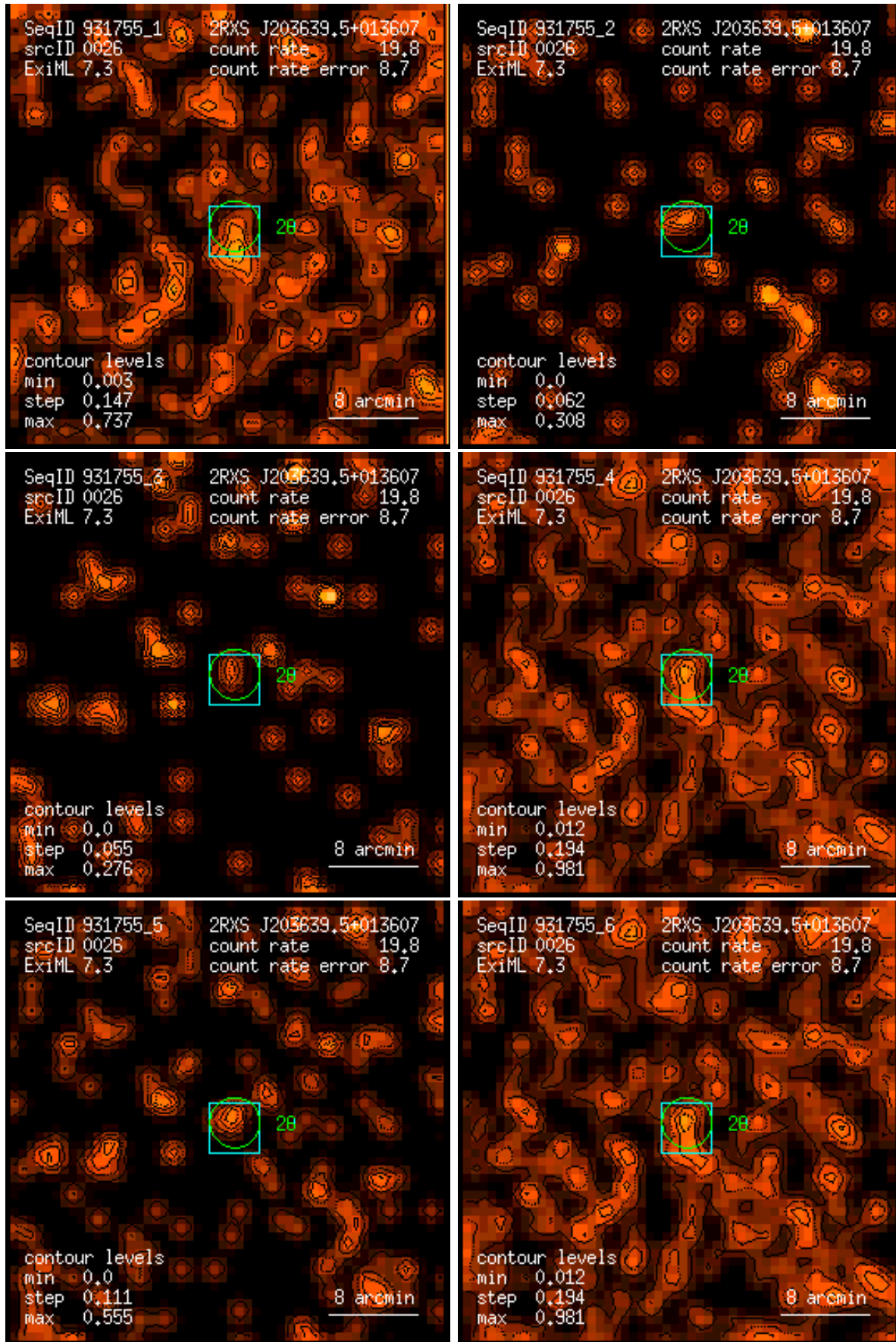
Figure 26: RASS 931755: detection 0026: band rate images, Gaussian filter: (1) PSPC channels 11 – 41, (2) 52 – 90, (3) 91 – 201, (4) 11 – 235, (5) 52 – 201, (6) 11 – 201. Broad band rates in counts/ks. Band rate contour levels in counts/ks/arcmin 2 .
