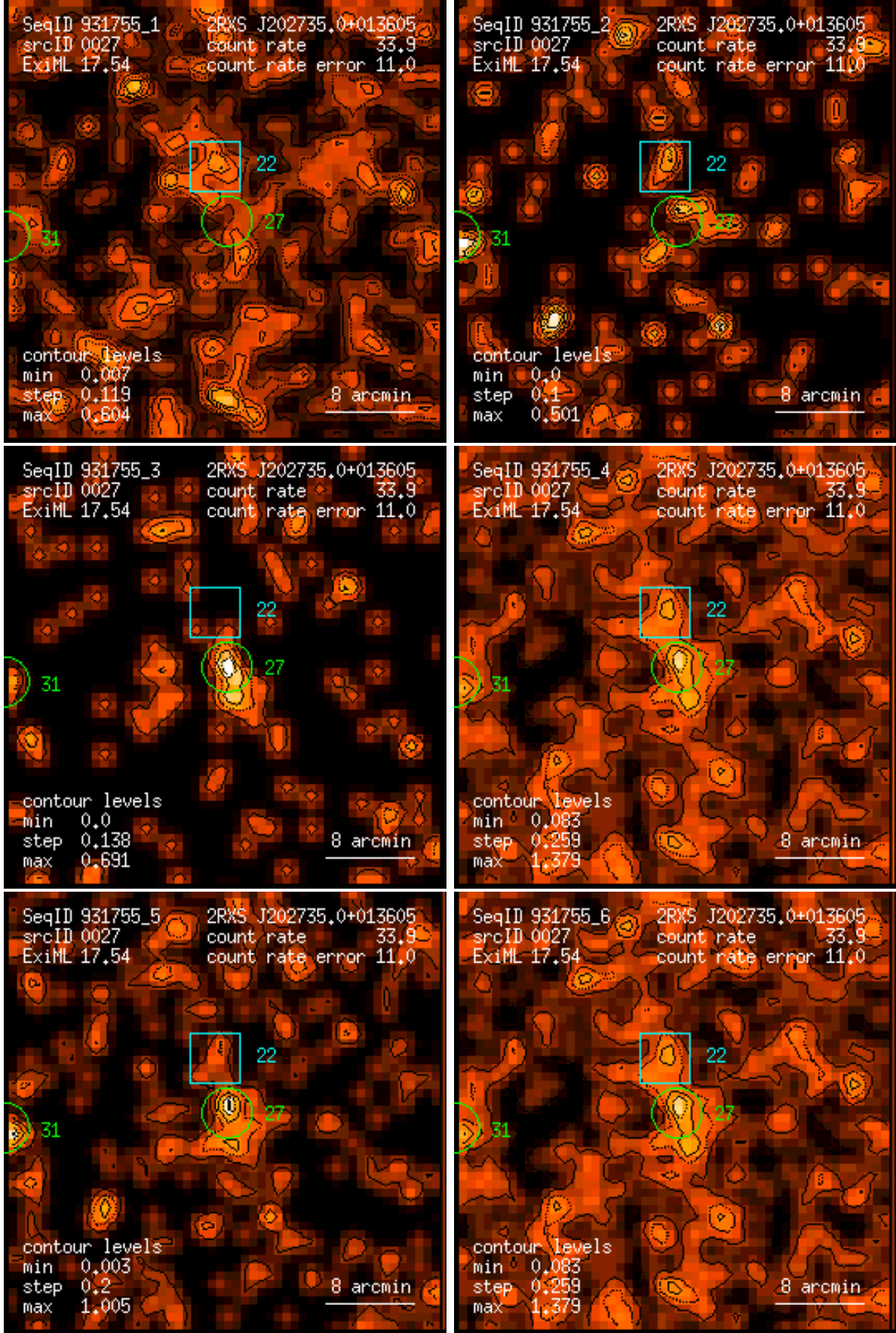
Figure 27: RASS 931755: detection 0027: band rate images, Gaussian filter: (1) PSPC channels 11 – 41, (2) 52 – 90, (3) 91 – 201, (4) 11 – 235, (5) 52 – 201, (6) 11 – 201. Broad band rates in counts/ks. Band rate contour levels in counts/ks/arcmin 2 .
