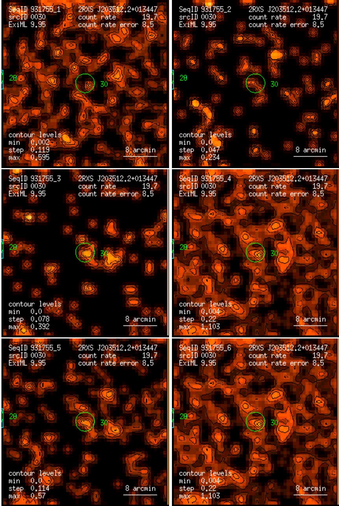
Figure 30: RASS 931755: detection 0030: band rate images, Gaussian filter: (1) PSPC channels 11 – 41, (2) 52 – 90, (3) 91 – 201, (4) 11 – 235, (5) 52 – 201, (6) 11 – 201. Broad band rates in counts/ks. Band rate contour levels in counts/ks/arcmin 2 .
