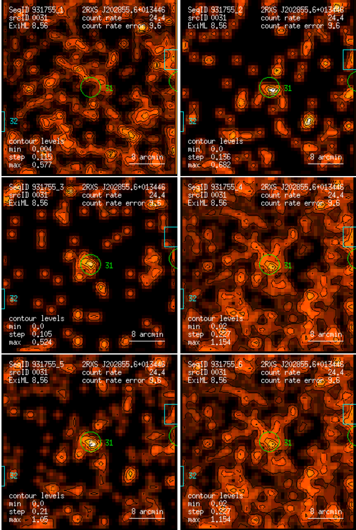
Figure 31: RASS 931755: detection 0031: band rate images, Gaussian filter: (1) PSPC channels 11 – 41, (2) 52 – 90, (3) 91 – 201, (4) 11 – 235, (5) 52 – 201, (6) 11 – 201. Broad band rates in counts/ks. Band rate contour levels in counts/ks/arcmin 2 .
