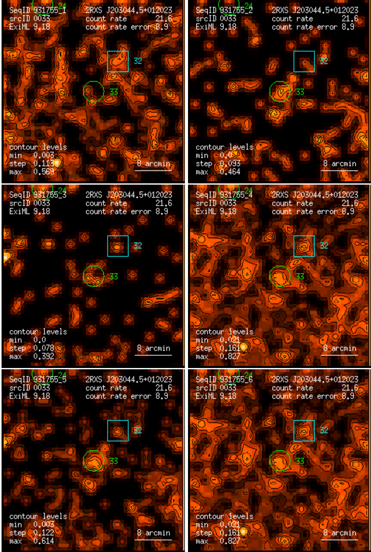
Figure 33: RASS 931755: detection 0033: band rate images, Gaussian filter: (1) PSPC channels 11 – 41, (2) 52 – 90, (3) 91 – 201, (4) 11 – 235, (5) 52 – 201, (6) 11 – 201. Broad band rates in counts/ks. Band rate contour levels in counts/ks/arcmin 2 .
